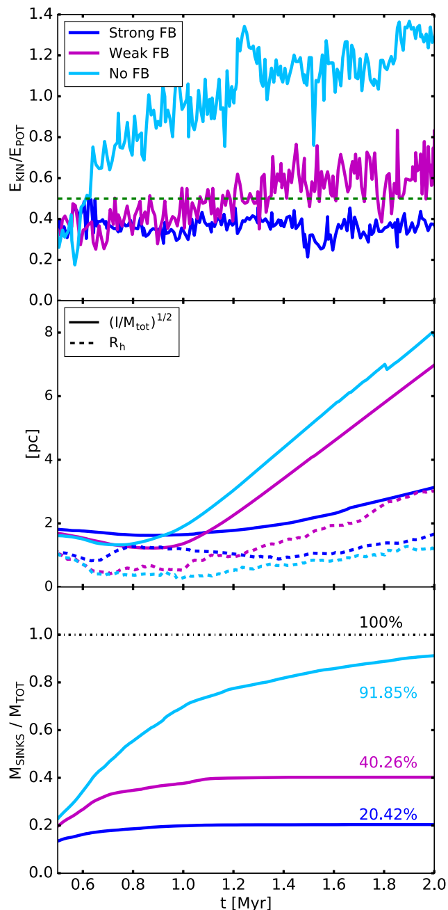
Figure 2. Top panel: ratio of total kinetic to potential energy of the sinks (virial ratio, E_k/E_p ), the dashed green line indicates the virial equilibrium. Middle panel: size of the star cluster, in terms of half-mass radius (dashed line) and moment of inertia-derived radius (solid line). I and M_{\text{SINKS}} indicate respectively the moment of inertia and total mass of sinks. Bottom panel: SFE evolution with time computed as the mass fraction in sinks ( M_{\text{SINKS}} indicates the total mass in sinks, M_{\text{TOT}} , the total initial mass of the gas cloud). The ionizing radiation suppresses the formation of stars by clearing gas out of the cloud, and it increases the virial stability of the emerging star cluster.
