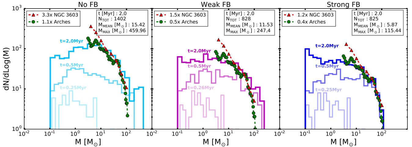
Figure 5. Mass function profile for all three feedback regimes. The thicker and darker lines indicate for every run the mass function profile at t = 2 Myr. In the top right box of every subplot, we indicated the total number of sinks, the average and maximum sink masses at t = 2 Myr. In every subplot, we plot also the mass functions at t = 0.5 Myr and t = 0.25 Myr in paler colours. The green dots correspond to the normalized observational data for the Arches cluster (Stolte et al. 2005), the red triangles the same for NGC 3603 (Pang et al. 2013). The normalization factors are reported in the top left box. Our strong feedback case compares best with the normalized observations, although all models fail to reproduce the steep curve towards lower masses in NGC 3603.
