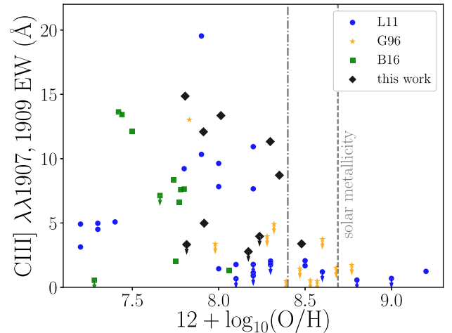
Figure 7. Equivalent width of the combined C III] \lambda\lambda 1907, 1909 semiforbidden doublet as a function of gas-phase metallicity. In addition to the HST/COS data presented in this paper, we plot archival data from nearby galaxies catalogued by Leitherer et al. (2011, L11), Giavalisco et al. (1996, G96) and Berg et al. (2016, B16) – see Appendix B for more details. These data suggest an empirical metallicity threshold for C III]: above 12 + \log O/H \sim 8.4 (marked by the dash-dotted line), C III] equivalent widths do not exceed \sim 5 Å. Below this threshold, extremely high equivalent widths \gtrsim 15 Å are achieved (comparable to that observed in the reionization era: Stark et al. 2015a, 2017), though not uniformly.
