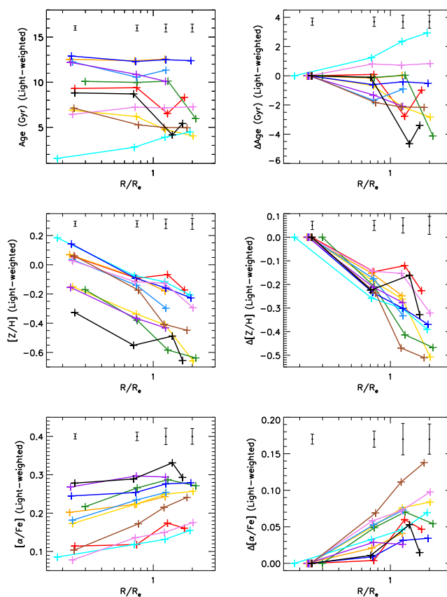
Figure 23. Absolute (left) and relative (right) profiles of light-weighted age (top), metallicity (middle) and [\alpha/\text{Fe}] abundance ratio, derived from PPF fits to combined spectra. Lines are as in Fig. 14. The black error bars show the mean error at a given aperture or annulus position.
