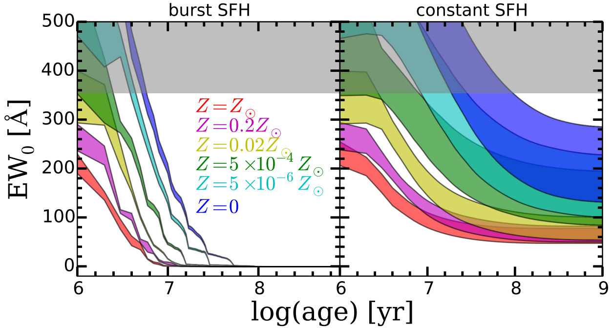
Fig. 12. Comparisons of the observational constraints on EW_0 with the models of Schaerer (2003) , Raiter et al. (2010) . These models show evolution of the spectral properties of stellar populations for stellar ages varying from 10^4 yr to 1 Gyr for the starburst SFH ( left panel ) and the constant SFH ( right panel ). Different colors correspond to six metallicities: Z = 0 (PopIII, blue), 5 \times 10^{-6} Z_\odot (cyan), 5 \times 10^{-4} Z_\odot (green), 0.02 Z_\odot (yellow), 0.2 Z_\odot (magenta), and Z_\odot (red). For each metallicity, the colored shaded regions denote EW_0 ranges traced by the three three power-law IMFs: two Salpeter IMFs ( 1-100 M_\odot and 1-500 M_\odot ) and a Scalo IMF ( 1-100 M_\odot ). The horizontal gray shaded regions indicate the range of nine very large EW_0 LAEs without signatures of mergers or AGNs.
