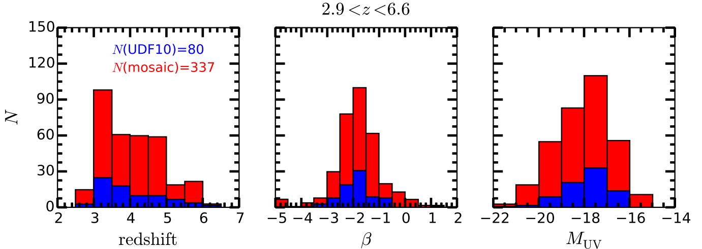
Fig. 1. Left, middle, and right panels: distributions of z , \beta and M_{UV} for the entire sample at 2.9 < z < 6.6 , respectively. In each panel, the blue and red histograms correspond to the distributions for udf-10 and mosaic, respectively. A two-sample Kolmogorov-Smirnov test (K-S test) results in the p -value of 0.84, 0.25, and 0.32 for the two z , \beta and M_{UV} distributions, respectively, indicating that the distributions of the values in the two fields cannot be distinguished from each other.
