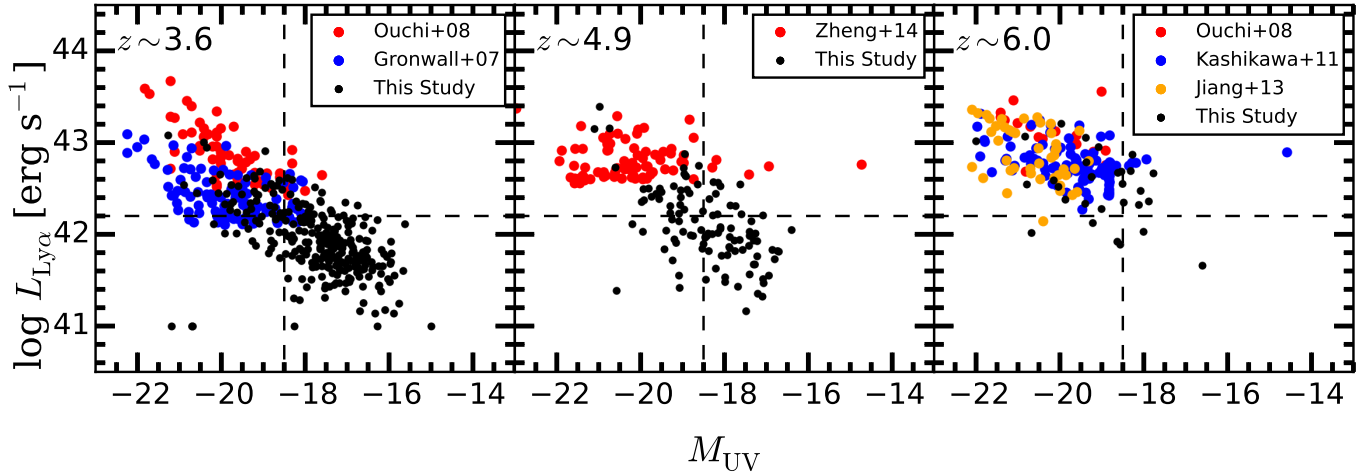
Fig. 6. From left to right: \log L_{\text{Ly}\alpha} plotted against M_{\text{UV}} for z \sim 3.6 , 4.9 , and 6.0 . The black circles indicate our individual LAEs. In each panel, objects with \log (L_{\text{Ly}\alpha}/\text{erg s}^{-1}) < 41.0 are placed at 41.0 for display purposes. Left panel: red circles show spectroscopically confirmed LAEs from Ouchi et al. (2008) at z \sim 3.1 and 3.7 , while blue circles indicate a photometric LAE sample from Gronwall et al. (2007). Middle panel: red circles correspond to z \sim 4.5 LAEs studied by Zheng et al. (2014). Right panel: red circles show spectroscopically confirmed LAEs from Ouchi et al. (2008) at z \sim 5.7 . Blue circles indicate spectroscopically confirmed LAEs from Kashikawa et al. (2011) at z \sim 5.7 and 6.5 , while orange circles are spectroscopically confirmed LAEs from Jiang et al. (2013) at z \sim 5.7 , 6.5 , and 7.0 . In each panel, the vertical dashed line at M_{\text{UV}} = -18.5 and the horizontal dashed line at \log (L_{\text{Ly}\alpha}/\text{erg s}^{-1}) = 42.2 show the cuts used for fair comparisons of EW_0 scale lengths at 2.9 < z < 6.6 (see Sect. 6.3).
