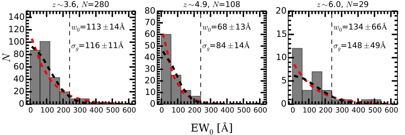
Fig. 7. From left to right: EW_0 distributions for z \sim 3.6 , 4.9 , and 6.0 with a bin width of 60 \text{ \AA} (gray histograms). One (one) object at z \sim 3.6 ( 4.9 ) with EW_0 > 600 \text{ \AA} is placed at EW_0 = 600 \text{ \AA} for display purposes. The vertical dashed line indicates EW_0 = 240 \text{ \AA} (cf. Schaerer 2003 ; Raiter et al. 2010 ). The red dashed lines show the best-fit curves of the distributions expressed as N = N_0 \exp(-EW_0/w_0) , where w_0 indicates the best-fit scale factor. The black dashed lines indicate the best-fit curves of the distributions expressed as N = N_0 \exp(-EW_0^2/2\sigma_g^2) , where \sigma_g indicates the best-fit distribution width.
