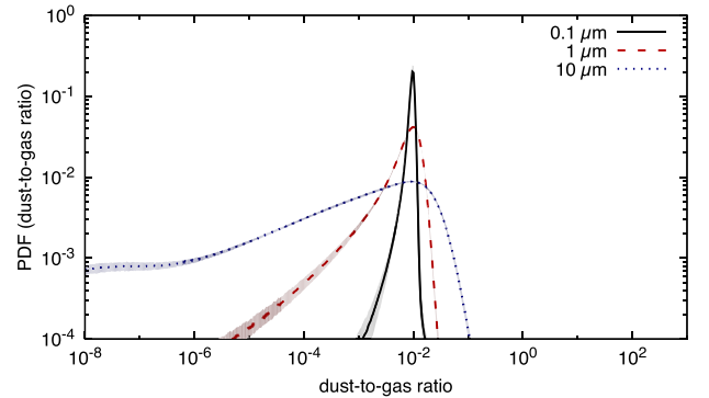
Figure 4. Time-averaged volume weighted PDFs of the dust-to-gas ratio. The dust-to-gas ratio for all grain sizes is peaked at 1 per cent. Minimal variation in the dust-to-gas ratio occurs for 0.1 \mu\text{m} grains, but the PDFs broaden with increasing grain size caused by size-sorting of large grains, meaning larger volumes of the cloud are either dust enriched or dust depleted.
