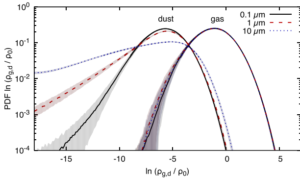
Figure 3. Time-averaged volume weighted PDFs of \ln(\rho_g/\rho_0) and \ln(\rho_d/\rho_0) . Shaded regions represent the standard deviation of the time averaging. The gas density is log-normal. Small, 0.1 \mu\text{m} dust grains show a log-normal PDF, mirroring the gas. Larger grains show a skewed distribution, with regions of both low- and high-dust densities being more common, indicating the preferential concentration of large grains into dense regions.
