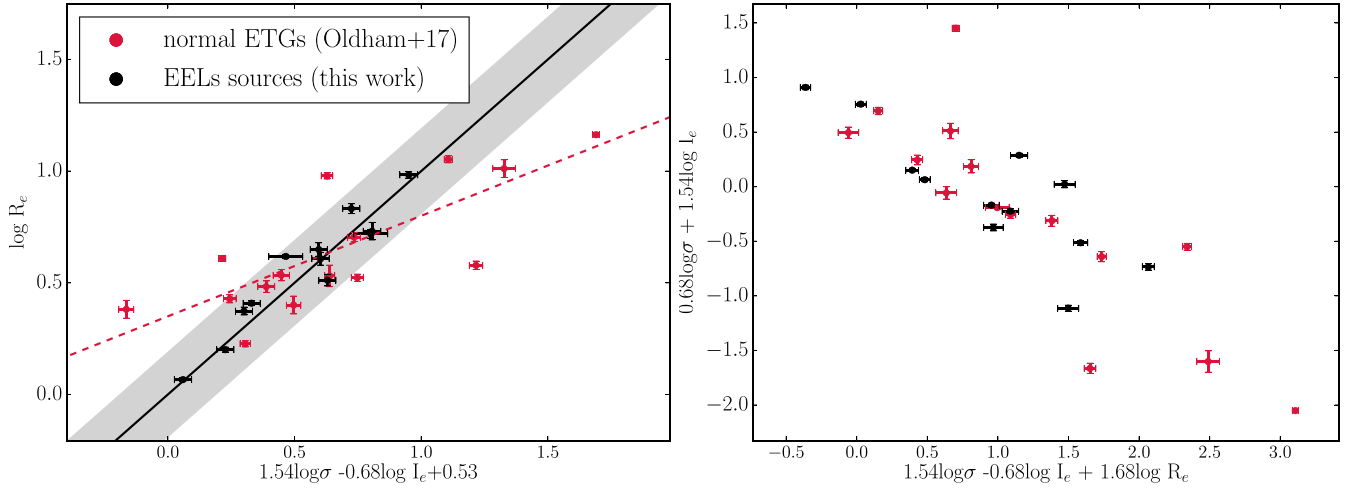
Figure 2. The observed FP of the massive compact EELs sources, shown in side-on (left) and face-on (right) projections, with the similar-redshift, less compact ETGs from Oldham, Houghton & Davies (2017b) shown in red for comparison. The FP is steeper in \log \sigma and shallower in \log I_e relative to that of the ‘normal’ Oldham et al. (2017b) galaxies, which indicates that both the dark and stellar mass structure and stellar populations vary as a function of the plane parameters. The FP also has a comparable intrinsic scatter to that of normal ETGs, implying that the intrinsic scatter is driven by stellar population properties. Velocity dispersions, surface brightnesses and effective radii are measured in units 200 \text{ km s}^{-1} , 10^9 L_{\odot} and kpc, respectively.
