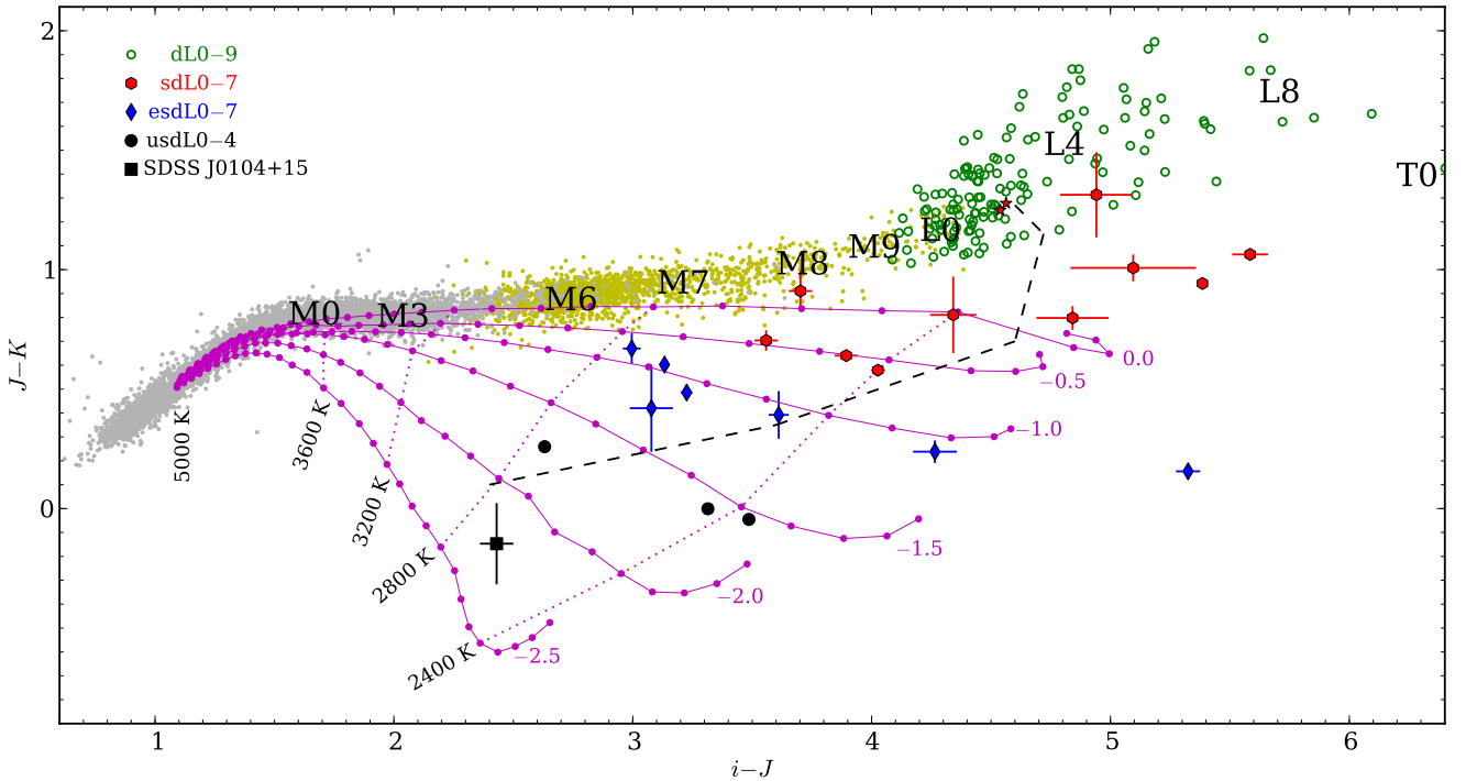
Figure 2. The i - J versus J - K colours of L subdwarfs compared to M and L dwarfs. Red hexagon, blue diamonds and black circles are sdL, esdL and usdL subdwarfs classified by Zhang et al. (2017). The three usdLs (black circles from left to right) are SSSPM J1013–13 (usdL0), SDSS J1256–02 (usdL3) and 2MASS J1626+39 (usdL4). The black square is SDSS J0104+15. Some objects do not show error bars because these are smaller than the symbol size. Grey dots are 5000 point sources selected from a 10 \text{ deg}^2 area of UKIDSS sky with 14 < J < 16 . Yellow dots are 1820 spectroscopically confirmed late-type M dwarfs (for which mean spectral types are indicated) from West et al. (2008). The BT-Settl model grids (Allard et al. 2014) with \log g = 5.5 (magenta) are overplotted for comparison, with T_{\text{eff}} (2000–5000 K) and [\text{Fe}/\text{H}] (from -2.5 to 0.0 ) indicated. Two five-pointed stars filled with red are the L1 SSSPM J0829–1309 and the L2.5 2MASS J0523–1403, which are likely least massive stars in the local field (Dieterich et al. 2014). They are not detected in SDSS and UKIDSS; therefore, PS1 i , and VHS J and K photometry are used. The difference between SDSS i and PS1 i -band photometry of L dwarfs is \sim \pm 0.05 . The black dashed broken line indicates the roughly stellar–substellar boundary. Note this boundary is based on observed colours of least massive stars and brown dwarfs, not based on model predicted colours.
