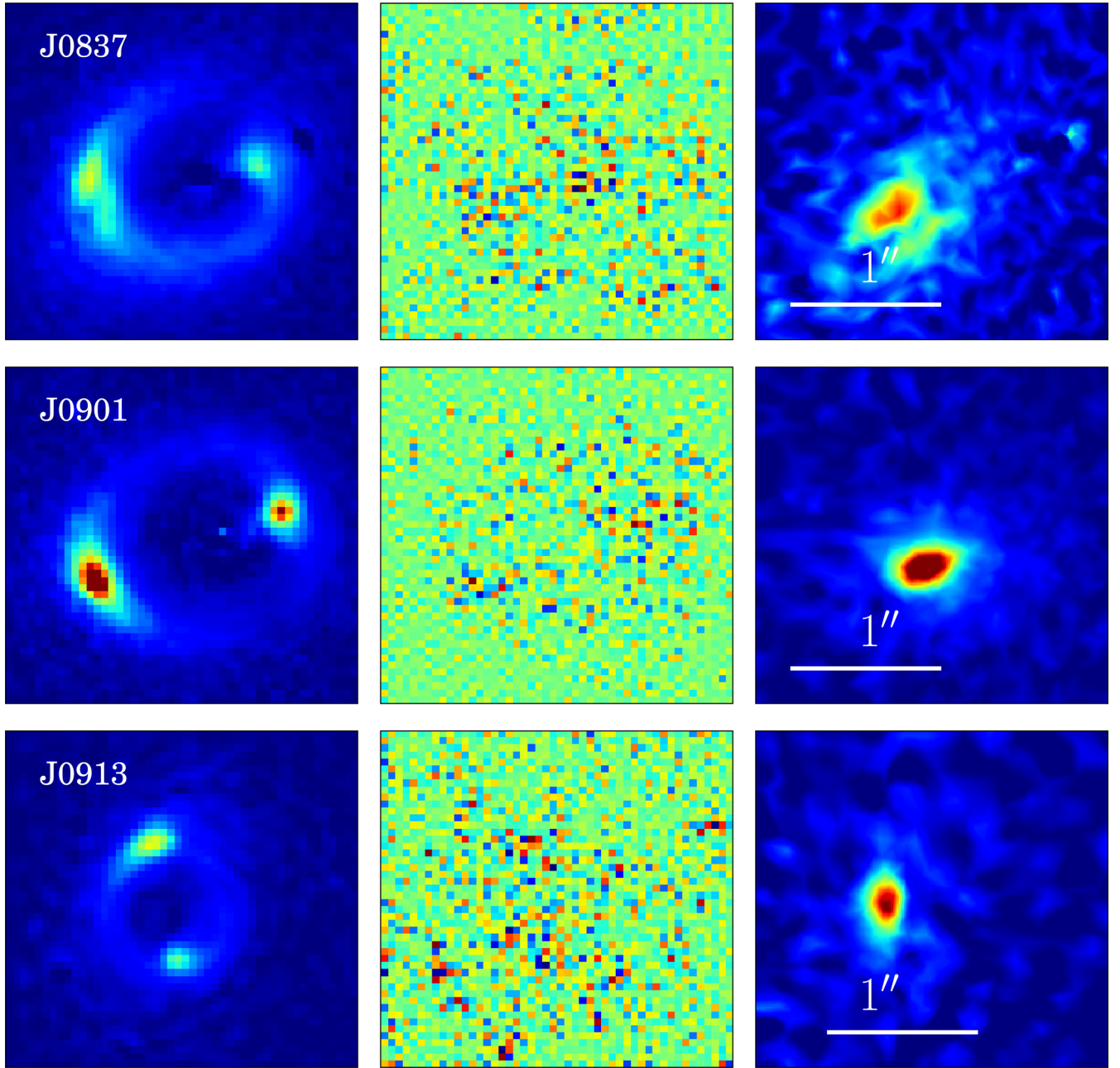
Figure A1. Pixellated reconstructions for the 13 EELs analysed here. From left to right, we show the V-band image, the signal-to-noise residuals and the reconstructed source. Note that these are not fitted models, but reconstructions of the source based on the lens models inferred using parametric source models. These reconstructions generally confirm that the sources are smooth, though they also recover the dust lane feature in J0837 and the disc features in J1446 and J1606.
