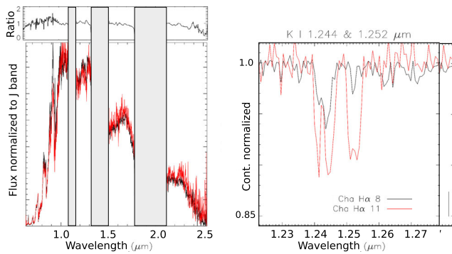
Figure 18. Left: direct comparison of the optical + near-infrared spectra of Cha H \alpha 8 (in black) and Cha H \alpha 11 (in red). Both spectra have been dereddened according to the A_V values given in Table 6 corresponding to the optical + NIR fitting approach. In the upper panel, the ratio between both spectra is provided. In both panels, the areas where we have not been able to correct for the strong telluric bands are covered with white rectangles. Right: detail of the continuum normalized spectra for both sources in the spectral region of the K I doublet analysed in Section 5. The colour code is the same as in the left-hand panel.
