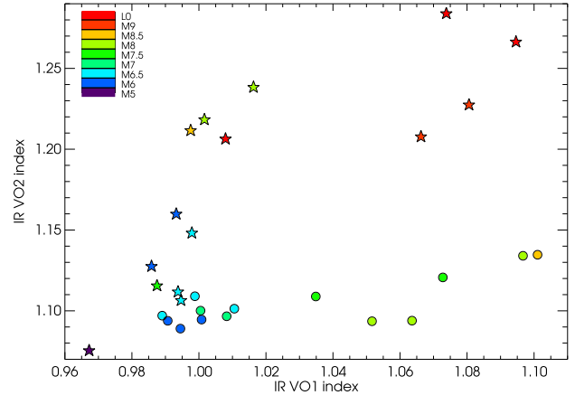
Figure 6. VO1 versus VO2 indexes for the sample of young (Cha I and TWA members, filled circles) and old (field dwarfs, filled stars) sources. All symbols are colour coded according to the spectral type of the object (see legend).
