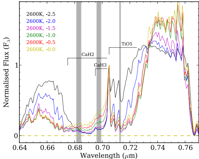
Figure 6. BT-Settl model spectra with an T_{\text{eff}} of 2600 K, and [\text{Fe}/\text{H}] of 0.0, -0.5 , -1.0 , -1.5 , -2.0 , and -2.5 (Allard et al. 2014). Shaded areas are explained in the caption to Fig. 5.
