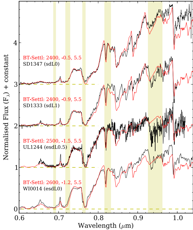
Figure 19. Optical spectra of four subdwarfs compared to the best-fitting BT-Settl models. T_{\text{eff}} , [\text{Fe}/\text{H}] , and \log g of the models are indicated. Spectra are normalized at 0.815 \mu\text{m} . Model spectra have a resolving power of 500 at 1 \mu\text{m} .
