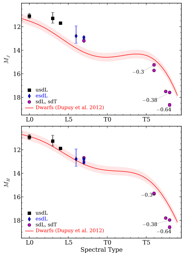
Figure 22. The relationship between spectral type and J - and H -band absolute magnitudes (MKO) for L and T subdwarfs. The red solid line is for M–L–T dwarfs (Dupuy & Liu 2012). The shaded area shows the fitting rms. Three numbers to the left of three sdT companions indicate that [\text{Fe}/\text{H}] was inferred from their bright primary stars (Cenarro et al. 2007; Rojas-Ayala et al. 2012; Pinfield et al. 2012). Note that sdL7 and sdT7.5 are components of a wide binary SD1416 AB. Error bars for some objects are similar to or smaller than the plotting symbols.
