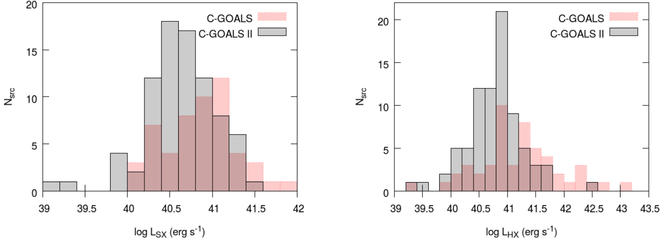
Fig. 7. Distributions of soft-band X-ray luminosity, 0.5–2 keV ( left panel ), and hard-band X-ray luminosity, 2–10 keV ( right panel ), for the individual galaxies of CGI and CGII.
