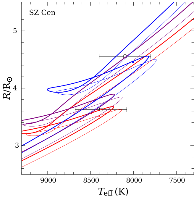
Fig. 1. Evolution tracks of stellar models of SZ Cen. Thick lines denote the primary models. Error bars indicate the uncertainty in R and T_{\text{eff}} reported by Torres et al. (2010) . The models have 0.013 \leq f_{\text{os}} \leq 0.028 and -0.25 \leq [\text{Fe}/\text{H}] \leq -0.20 . The redder curves show models with lower f_{\text{os}} .
