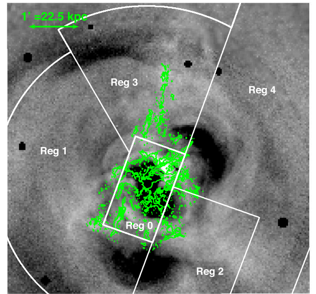
Figure 4. Chandra composite fractional residual image from Fabian et al. (2011) in the 0.5–7keV band (1.4 Ms exposure). The point spread function (PSF) corrected Hitomi regions from Hitomi Collaboration et al. (2017) are shown in white. Contours from the H\alpha flux map (starting at 3 \times 10^{-17} \text{ erg/s/cm}^2/\text{pixel} ) are shown in green.
