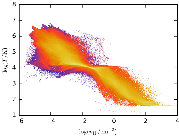
Figure 1. Phase diagram of the gas within the virial radius of an M_{\text{H}} = 10^{10.5} M_{\odot} halo at z = 3 , simulated with supernova feedback. Gas considered gravitationally bound to satellites has been removed. The colour scheme is scaled logarithmically with the gas mass enclosed in each pixel, ranging from blue at low enclosed mass to yellow-white at high enclosed mass.
