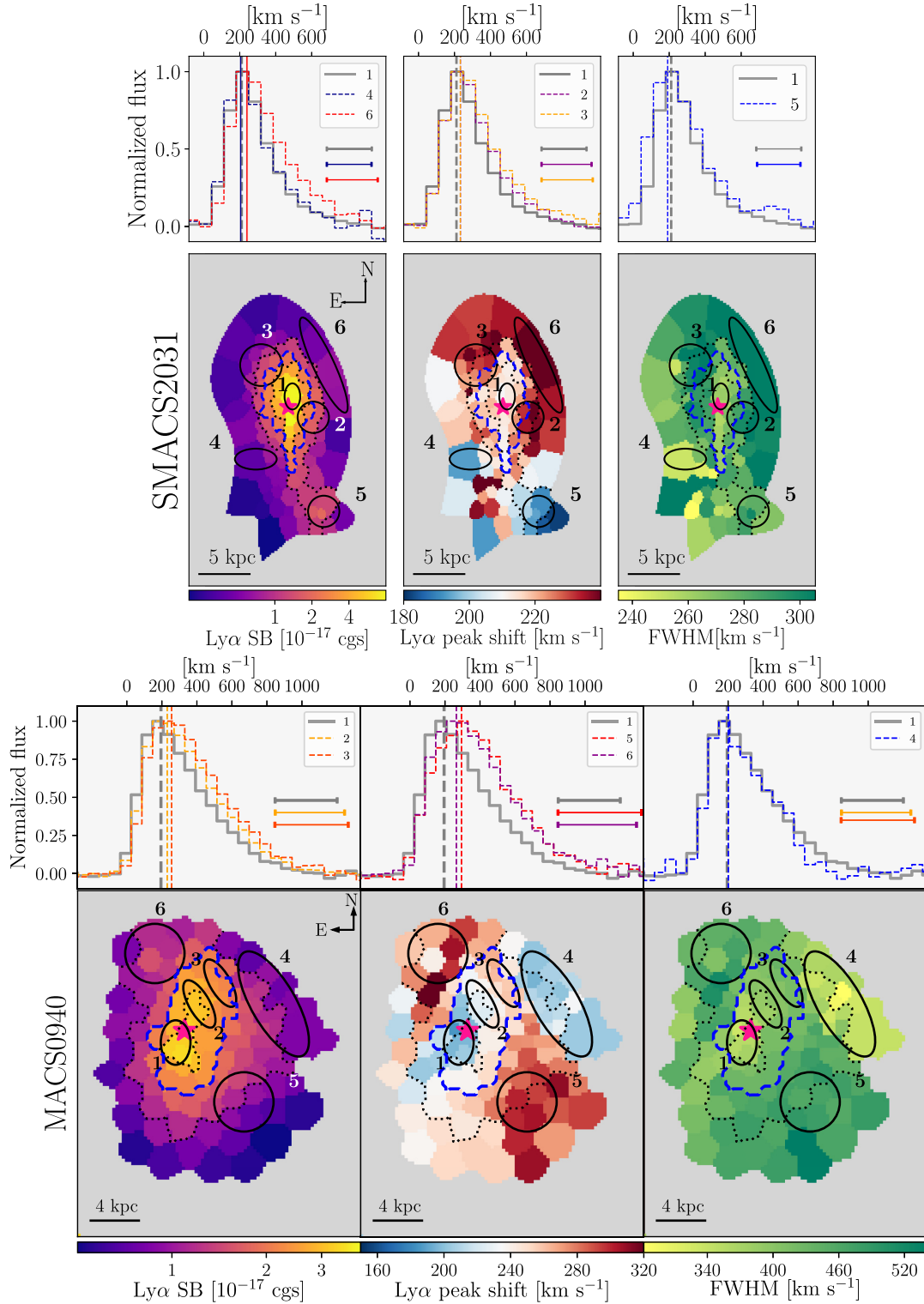
Figure 2. Lyman \alpha spectral line analysis for SMACS2031 (upper panel) and MACS0940 (lower panel) in the source plane. For each object, top: spectra of specific regions of the halo (indicated by black ellipses on maps). The vertical lines represent the position of the peak wavelength produced by the asymmetric fit. Horizontal segments represent the FWHM of each line. Bottom left: maps of the Lyman \alpha SB profile in the halo. Middle: map of the Lyman \alpha peak shift relative to the systemic redshift. Bottom right: map of the FWHM in the halo. In all bottom panels: dashed lines represent SB isocontours at 1, 2, and 3 \times 10^{-17} erg s ^{-1} cm ^{-2} arcsec ^{-2} . The blue contour corresponds to the SB threshold used in Fig. 4, i.e. 2 \times 10^{-17} erg s ^{-1} cm ^{-2} arcsec ^{-2} . The pink star marks the position of the peak of the stellar UV continuum.
