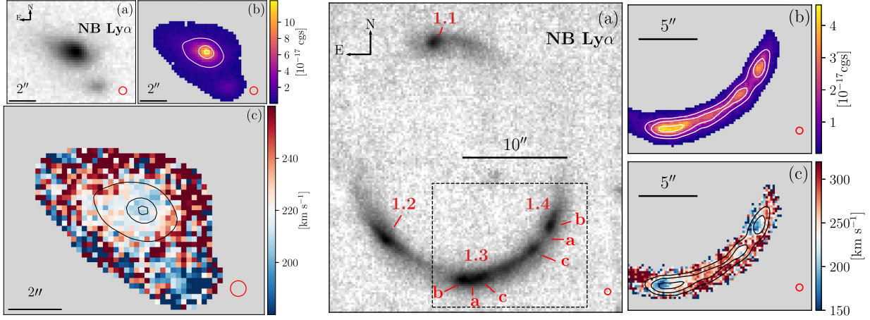
Figure 1. NB Lyman \alpha image and pixel-by-pixel Lyman \alpha analysis in the image plane for SMACS2031 (left-hand panel) and MACS0940 (right-hand panel). For each panel: (a) NB Lyman \alpha image of the entire arc (MACS0940, labels mark the multiple systems presented in the Table A2) and only one image of SMACS2031 (image 1.3 according to the notation used in Richard et al. 2015), results of the individual spaxel fits [Lyman \alpha SB level (b) and peak shift (c)] for the most magnified images. The red circles show the MUSE PSF, and we overplot SB isocontours to highlight the flux peaks. The dashed grey box in panel (a) for MACS0940 represents the field of view of the two maps for this object.
