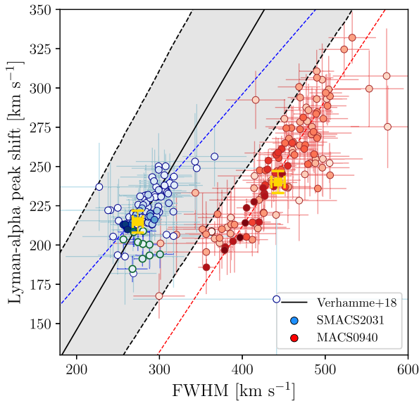
Figure 3. Lyman \alpha peak shift versus FWHM of the line in individual bins. Points are colour coded in intensity according to the line SB. The green circles are regions from the companion in the SMACS2031 galaxy. Yellow crosses indicate the values obtained for the fit to the total Lyman \alpha spectrum. The black solid line and shaded region represent the linear relation and errors found by Verhamme et al. (2018). The best-fitting parameters of this relation are presented in Table 1.
