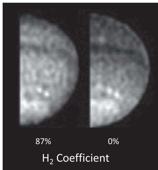
Fig. 1. Reproduction of part of Fig. 5 of Karkoschka and Tomasko (2011) showing HST/STIS observations of Neptune made in 2003 at two wavelengths near the 825 nm \text{H}_2\text{-H}_2/\text{H}_2\text{-He} CIA band, one where \text{H}_2\text{-H}_2/\text{H}_2\text{-He} opacity accounts for 87% of the opacity (left) and one where the opacity is entirely from gaseous methane (right). The images here have been processed to remove discrete features (Karkoschka and Tomasko, 2011). At wavelengths of low \text{H}_2\text{-H}_2 and \text{H}_2\text{-He} absorption (i.e. right) we see that the polar latitudes appear to be brighter than equatorial ones. If methane abundance were assumed to be constant with latitude, the brighter appearance of polar latitudes in the methane-image could be interpreted as being due to higher clouds there. However, the more uniform brightness seen in the \text{H}_2\text{-H}_2/\text{H}_2\text{-He} -absorbing image (left) shows that the appearance of Neptune in the methane-absorbing images is actually due to lower methane abundance at polar latitudes.
