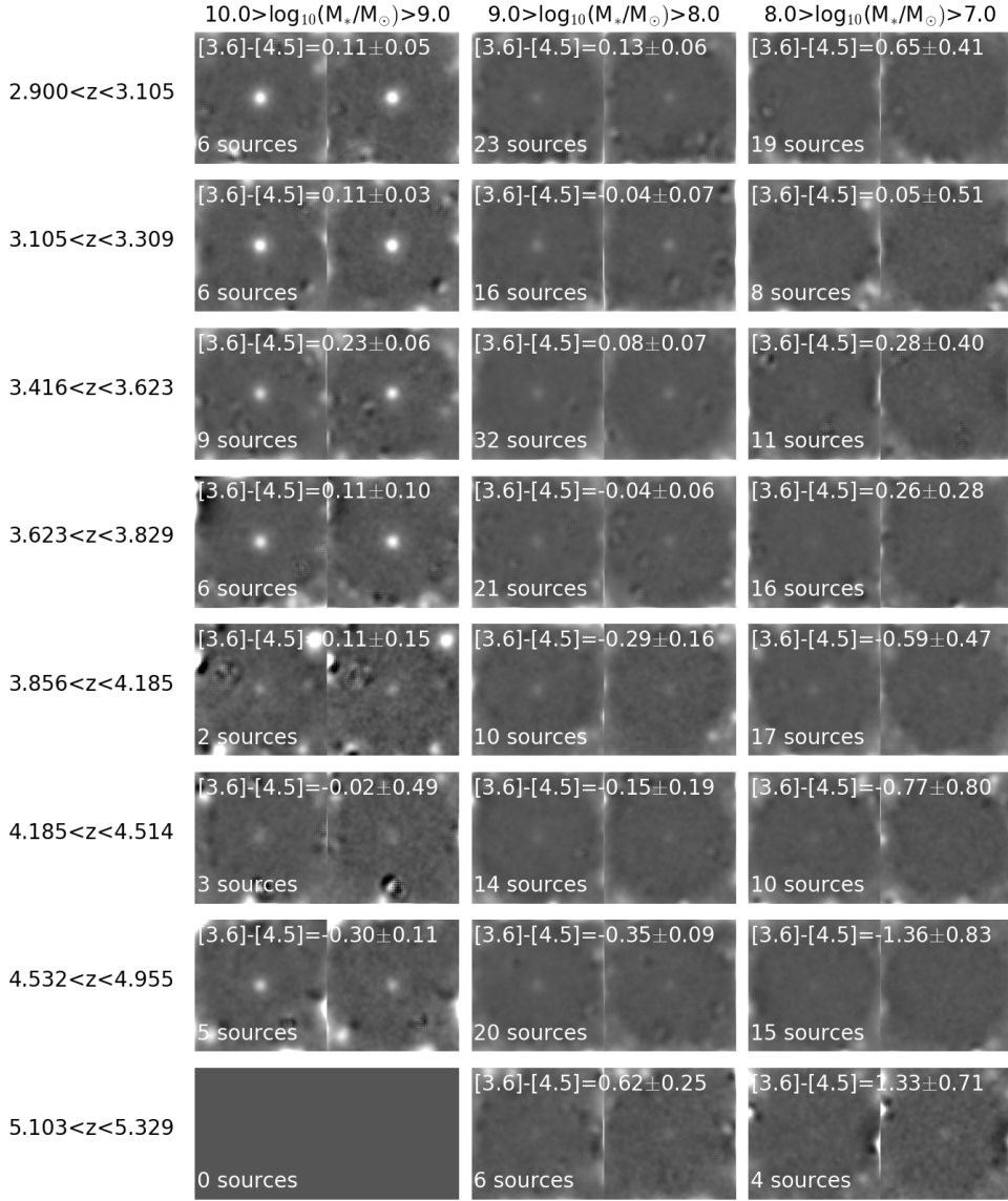
Fig. 6. Stacked Spitzer /IRAC [3.6] ( left ) and [4.5] ( right ) images of sources vs. their estimated stellar mass in the same redshift intervals considered in Fig. 5. Three different bins in stellar mass are considered: 10.0 < \log_{10}(M_*/M_\odot) < 9.0 , 9.0 < \log_{10}(M_*/M_\odot) < 8.0 , and 8.0 < \log_{10}(M_*/M_\odot) < 7.0 .
