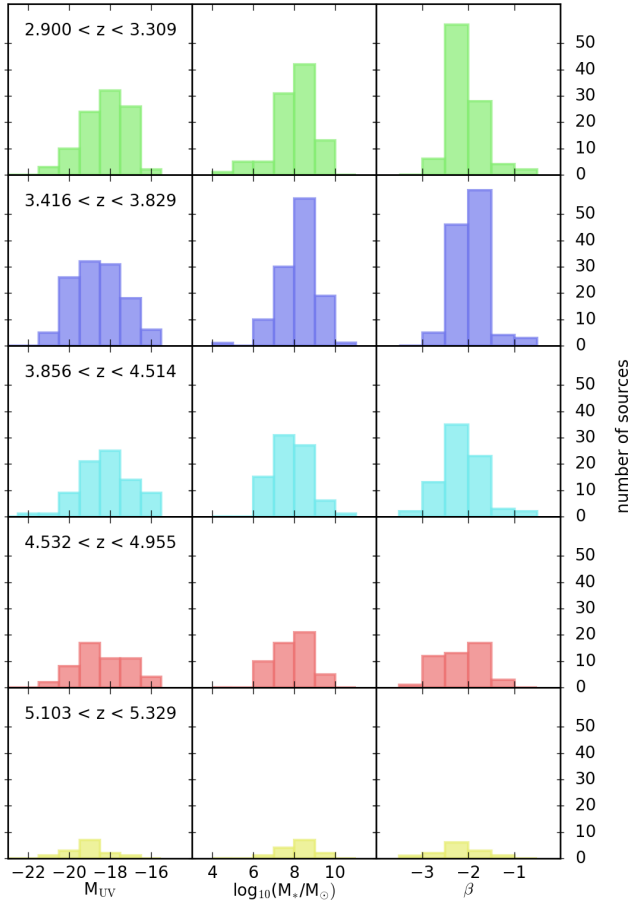
Fig. 4. Number of sources in each of the spectroscopic redshift intervals as a function of their absolute magnitudes (left column), stellar masses (middle column), and UV continuum slopes (right column). In estimating the strength of the H \alpha and [S III] lines, we make use of stacks of the Spitzer /IRAC images of the sources from each bin.
