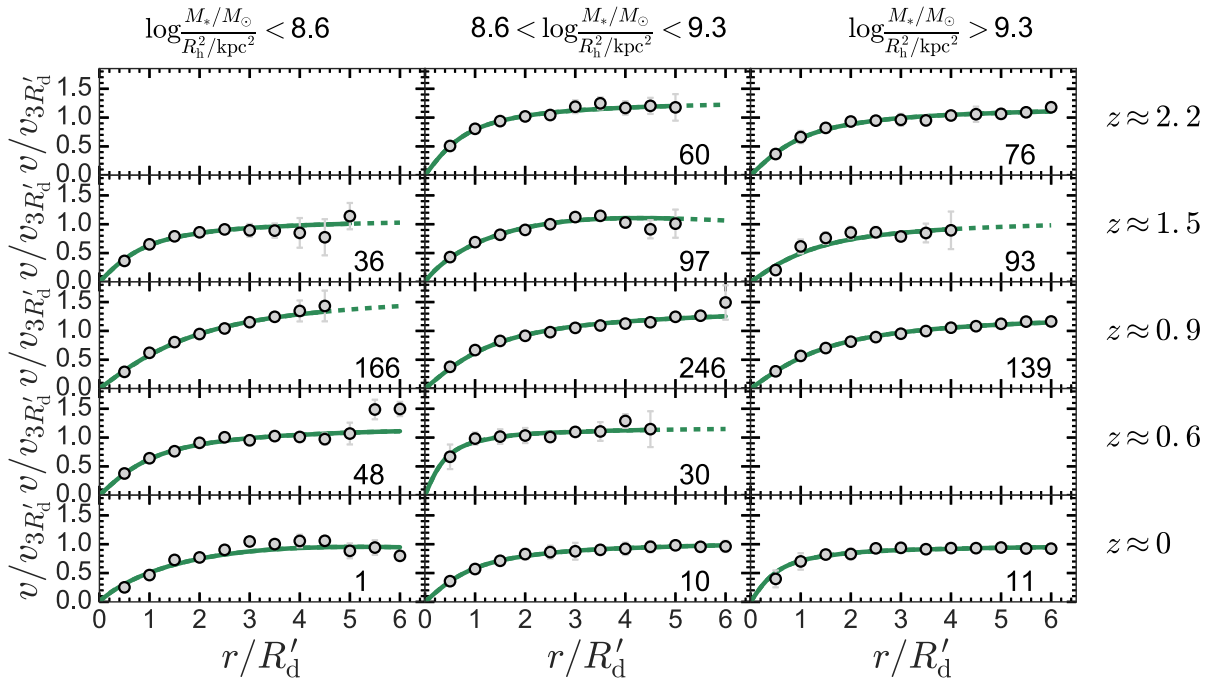
Figure 10. Average wrapped, normalized rotation curves for samples of galaxies from our analysis as a function of redshift (vertical) and central stellar mass density (horizontal). The rotation curves were constructed in the same manner as for Fig. 6. The green solid line in each panel represents the best-fitting model curve. The line is dashed when the model is extrapolated beyond the data. For all bins, the rotation curves either remain approximately flat or continue to rise out to the maximum radius probed in each case.
