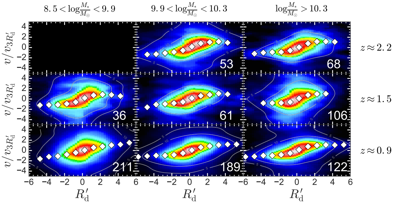
Figure A7. Median-averaged normalized position-velocity diagrams for samples of galaxies from our analysis separated into bins of redshift and mass. The position-velocity diagrams are derived from stacked H \alpha emission. We overlay grey contours corresponding to a signal-to-noise ratio of 5 and 10. The white diamonds in each panel represent the peak position of the best fit to the spectrum corresponding that radial column. The majority of the curves remain flat or continue to rise out to large radii.
