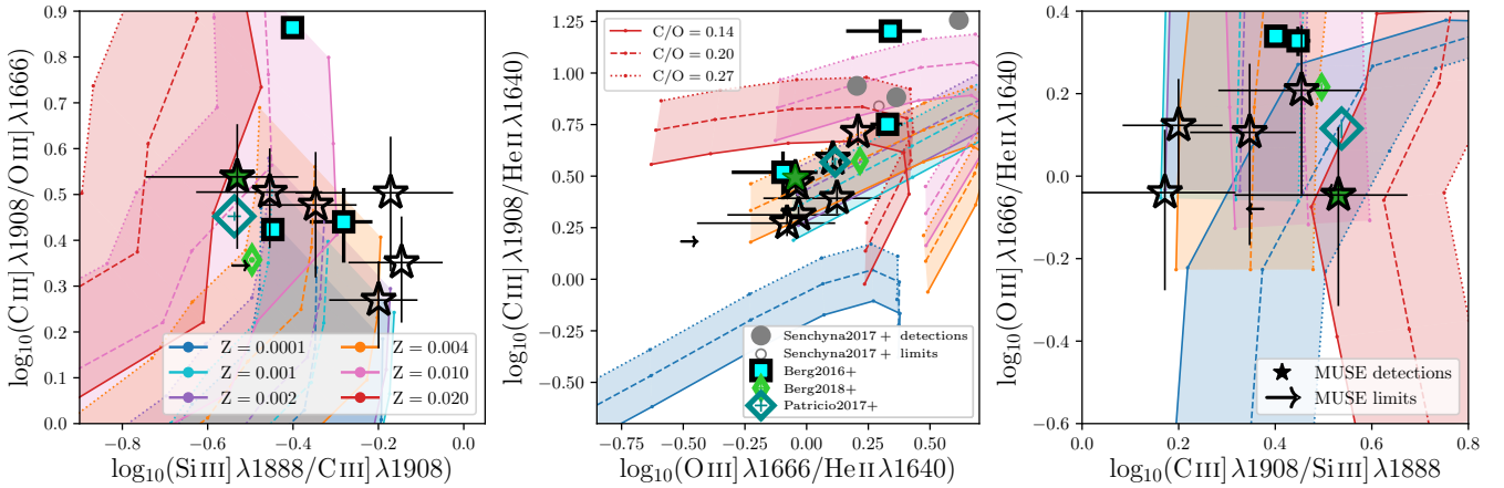
Fig. 6. Rest-frame UV emission line ratios of the MUSE He II \lambda 1640 sample. Left panel: C III]/O III] vs. Si III]/C III] ratios. Individual galaxies with S/N > 2.5 for all four emission lines are shown as stars. Limits are shown as arrows. The tracks are from the Gutkin et al. (2016) models, which are powered by star-formation. Each set of tracks with the same colour show three C/O ratios, and the regions between the minimum and maximum C/O tracks are shaded by the same colour. From top to bottom, the ionisation parameter increases. Where available, line ratios from Patricio et al. (2016), Senchyna et al. (2017), and Berg et al. (2018) are shown for comparison. MUSE line ratios of the Lyman continuum emitting candidate from Naidu et al. (2017) are shown by the filled green star. Centre panel: similar to the left panel, but C III]/He II \lambda 1640 vs. O III]/He II \lambda 1640 emission line ratios, where detections are defined as galaxies with S/N > 2.5 for all three emission lines. Right panel: similar to the left panel, but O III]/He II \lambda 1640 vs. C III]/Si III] emission line ratios, where detections are defined as galaxies with S/N > 2.5 for all four emission lines.
