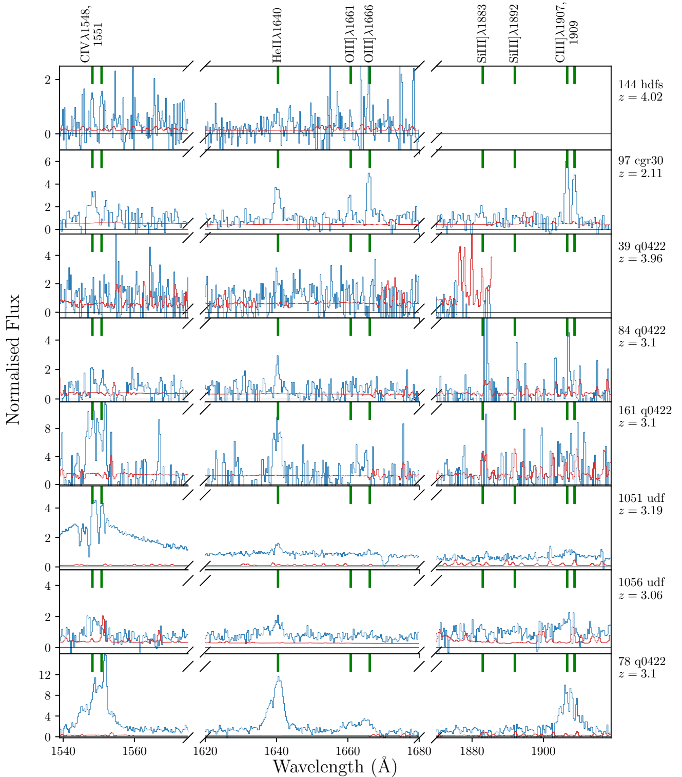
Fig. 2. continued. The last three panels show the spectra dominated by AGN activity.
