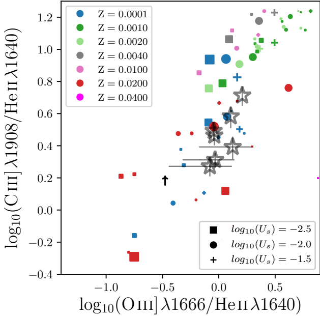
Fig. 8. Rest-frame UV emission line ratios of the MUSE He II \lambda 1640 sample compared with the model line ratios computed by Xiao et al. (2018) using BPASS binary stellar population models. Here we show the C III] \lambda 1908 /He II \lambda 1640 vs. O III] \lambda 1666 /He II \lambda 1640 line ratios for the MUSE He II \lambda 1640 detected sample. Individual galaxies with S/N \geq 2.5 for all three emission lines are shown as stars. Galaxies that fail the S/N cut are shown as arrows. The symbol size is proportional to the age from the onset of the star formation burst between t = 1 Myr (smallest) and t = 50 Myr. Models are computed with \log_{10}(n_{\text{H}}) = 1.0 with varying U_s between -2.5 and -1.5 . BPASS Z_{\odot} = 0.02 .
