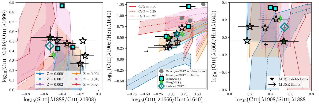
Fig. 6. Rest-frame UV emission line ratios of the MUSE He II \lambda 1640 sample. Left panel: C III]/O III] vs. Si III]/C III] ratios. Individual galaxies with S/N > 2.5 for all four emission lines are shown as stars. Limits are shown as arrows. The tracks are from the Gutkin et al. (2016) models, which are powered by star-formation. Each set of tracks with the same colour show three C/O ratios, and the regions between the minimum and maximum C/O tracks are shaded by the same colour. From top to bottom, the ionisation parameter increases. Where available, line ratios from Patricio et al. (2016), Senchyna et al. (2017), and Berg et al. (2018) are shown for comparison. MUSE line ratios of the Lyman continuum emitting candidate from Naidu et al. (2017) are shown by the filled green star. Centre panel: similar to the left panel, but C III]/He II \lambda 1640 vs. O III]/He II \lambda 1640 emission line ratios, where detections are defined as galaxies with S/N > 2.5 for all three emission lines. Right panel: similar to the left panel, but O III]/He II \lambda 1640 vs. C III]/Si III] emission line ratios, where detections are defined as galaxies with S/N > 2.5 for all four emission lines.
