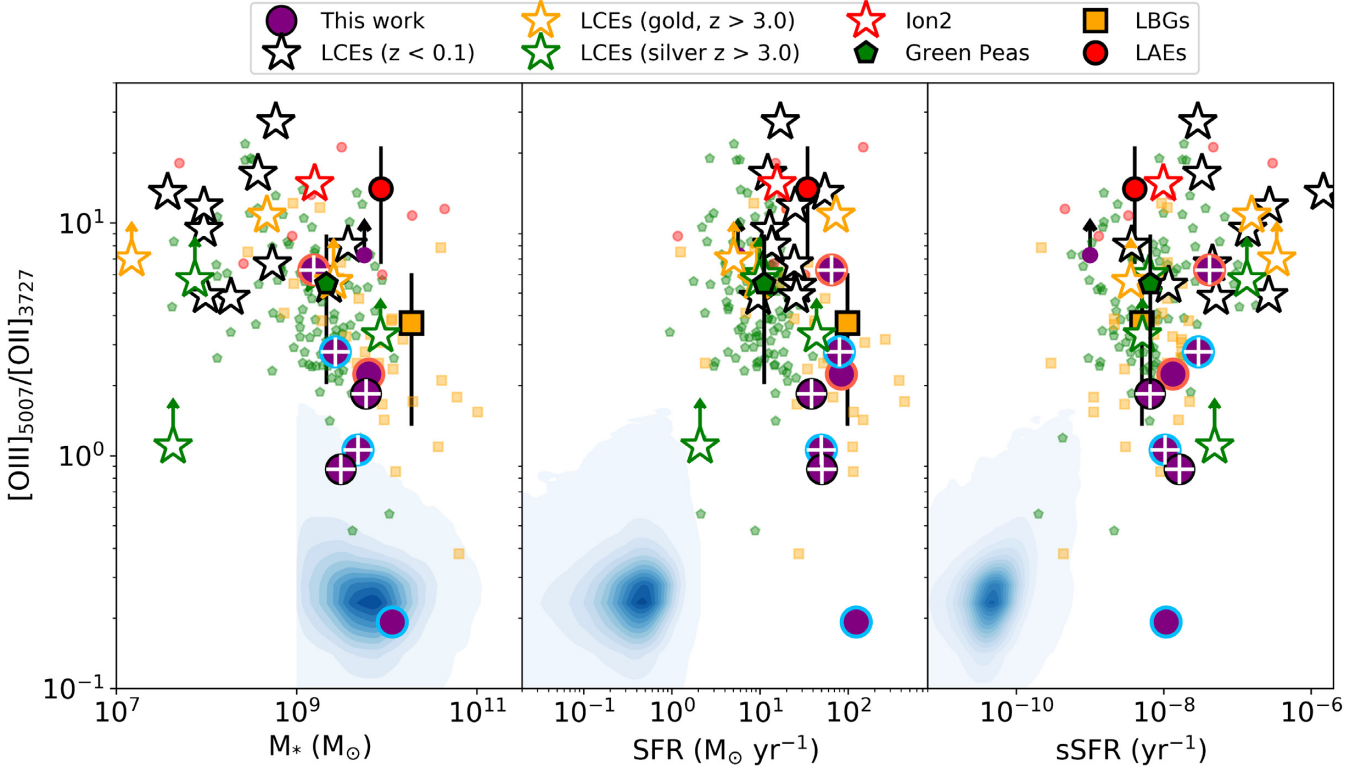
Figure 9. O32 as a function of M_* , SFR, and sSFR for galaxies in our MOSFIRE sample as well as low and high redshift comparison samples. Plotted symbols are the same as in Fig. 6. Purple circles with blue borders indicate the three galaxies having u -band flux consistent with f_{\text{esc}}(\text{LyC}) > 0.0 as estimated in Section 4.4. The two purple circles with red borders indicate galaxies where upper limits on u -band flux provide non-zero upper limits on f_{\text{esc}}(\text{LyC}) . The remaining three purple circles are galaxies where f_{\text{esc}}(\text{LyC}) is consistent with zero even within the photometric uncertainty. Galaxies in our sample have M_* comparable to low mass LBGs and high mass green peas, though up to 1 dex more massive than confirmed high- z LCEs. These results are likely reflective of relatively high stellar mass limits imposed for reliable photometric detections at high redshift (i.e. our desire to target bright galaxies). SFRs of our sample are comparable to LBGs, which are typically more star forming than green peas and LCEs. Finally, in terms of sSFR, galaxies in our sample are quite similar to confirmed LCEs.
