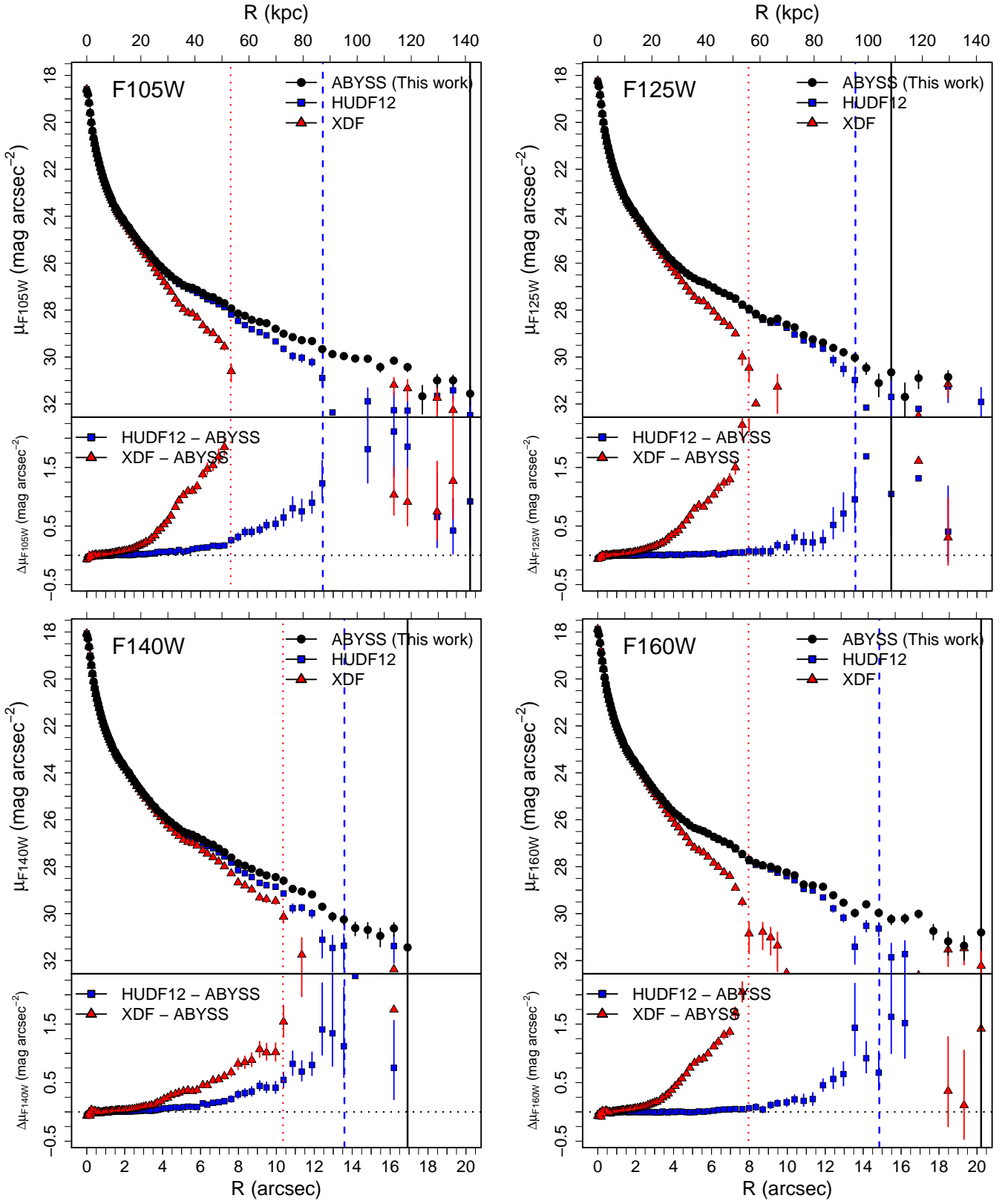
Fig. 20. Comparison of the surface brightness profiles of the elliptical galaxy HUDF-5 ( \alpha = 53.15545, \delta = -27.79150 , Buitrago et al. 2017) for the F105W (top left panel), F125W (top right panel), F140W (bottom left panel) and F160W filters (bottom right panel), using our own reduction of the HUDF WFC3 mosaics (ABYSS, black dots), the HUDF12 (Koekemoer et al. 2012, blue squares) and the XDF (Illingworth et al. 2013, red triangles). The top plot of each panel shows the surface brightness profile for each reduction. Black solid, blue dashed and red dotted lines represent the elliptical aperture with largest semi-major axis that presents an S/N higher than 3 over the sky-level. The bottom plot represents the difference in magnitude of each previous reduction with the ABYSS version of the mosaics as a function of galactocentric radius. Consult the legend on the figure.
