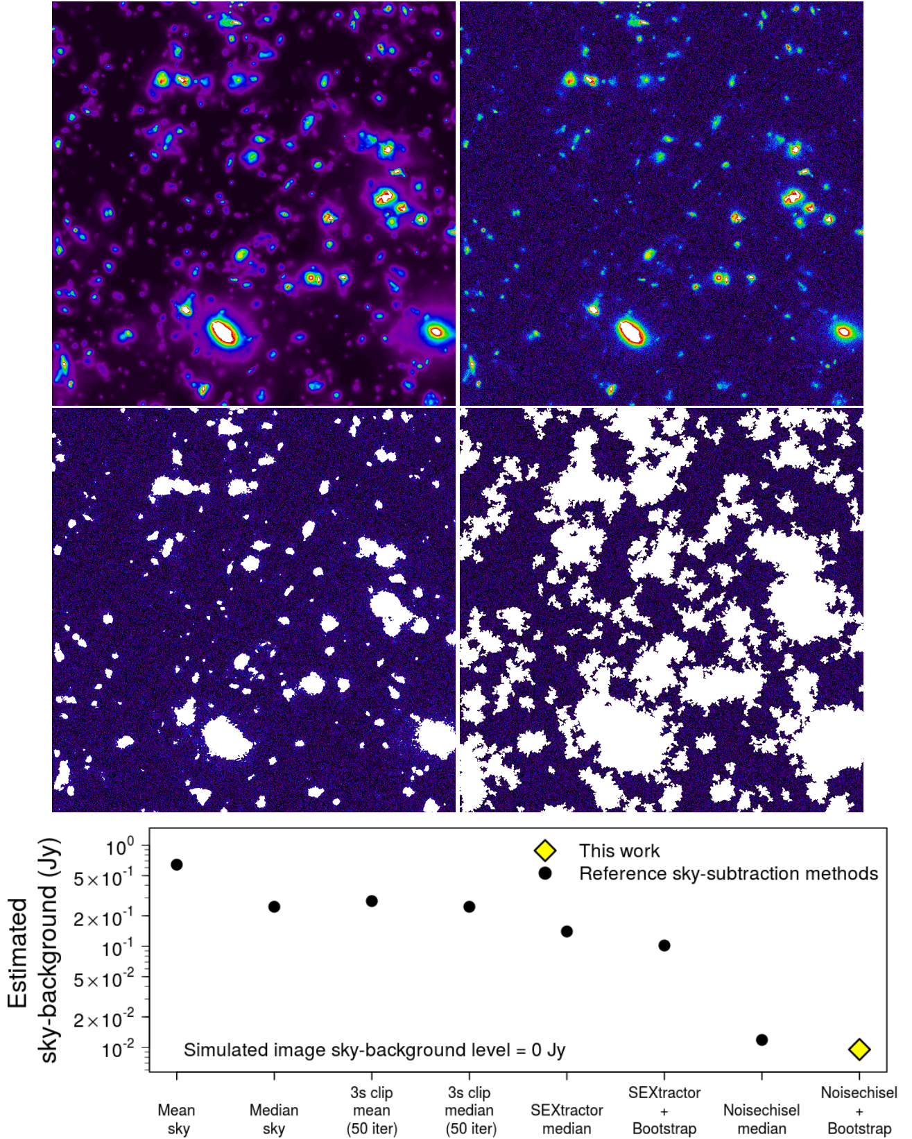
Fig. 9. Comparison of sky-subtraction methods, over a section of the Illustris simulation images. Top-left panel: simulated Illustris Deep Field B section. Top-right panel: same image with a 1 Jy wide Poissonian noise added. Middle-right panel: simulated Illustris Deep Field B with noise masked with SEXtractor ( 1\sigma threshold level). Middle-left panel: same image masked with NoiseChisel (default configuration). Bottom panel: estimated sky background as a function of different methods. Black dots: reference methods. Yellow diamond: method applied in the present paper. Notice that all methods overestimate the true sky background level, which is equal to zero in the simulated image. See the legend and axis for details.
