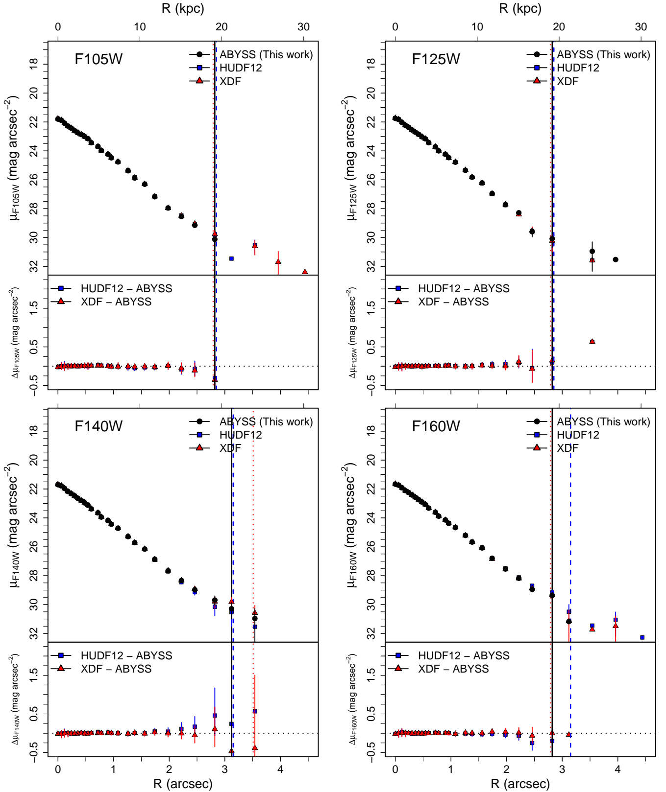
Fig. A.5. Comparison of the surface brightness profiles of the spiral galaxy ABYSS-3 ( \alpha = 53.15815 , \delta = -27.78109 , Elmegreen et al. 2005) for the F105W (top left panel), F125W (top right panel), F140W (bottom left panel), and F160W filters (bottom right panel), using our own reduction of the HUDF WFC3 mosaics (ABYSS, black dots), the HUDF12 (Koekemoer et al. 2012, blue squares), and the XDF (Illingworth et al. 2013, red triangles). The top plot of each panel shows the surface brightness profile for each reduction. Black solid, blue dashed, and red dotted lines represent the elliptic aperture with largest semi-major axis that presents an S/N higher than 3 over the sky-level. The bottom plot represents the difference in magnitude of each previous reduction with the ABYSS version of the mosaics as a function of galactocentric radius. Consult the legend on the figure.
