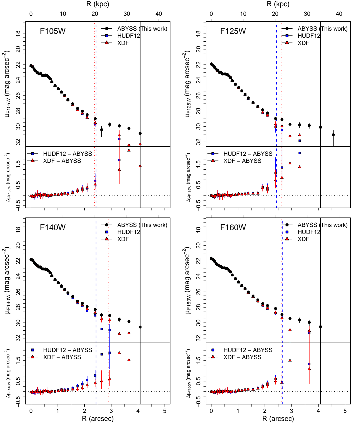
Fig. A.4. Comparison of the surface brightness profiles of the spiral galaxy ABYSS-2 ( \alpha = 53.17606 , \delta = -27.77371 , Elmegreen et al. 2005) for the F105W (top left panel), F125W (top right panel), F140W (bottom left panel), and F160W filters (bottom right panel), using our own reduction of the HUDF WFC3 mosaics (ABYSS, black dots), the HUDF12 (Koekemoer et al. 2012, blue squares), and the XDF (Illingworth et al. 2013, red triangles). The top plot of each panel shows the surface brightness profile for each reduction. Black solid, blue dashed, and red dotted lines represent the elliptic aperture with largest semi-major axis that presents an S/N higher than 3 over the sky-level. The bottom plot represents the difference in magnitude of each previous reduction with the ABYSS version of the mosaics as a function of galactocentric radius. Consult the legend on the figure.
