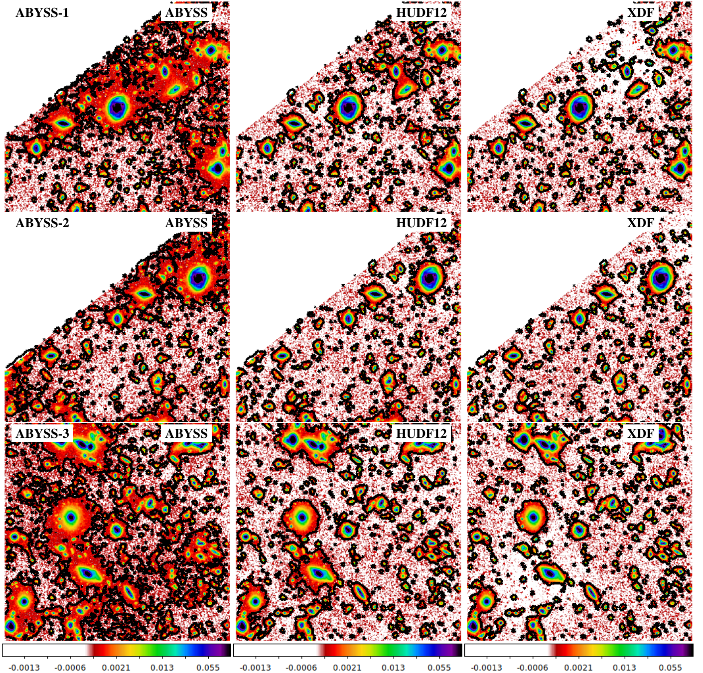
Fig. 19. F105W intensity images of ABYSS-1 (top row), ABYSS-2 (central row), and ABYSS-3 (bottom row) for our version of the HUDF mosaics (ABYSS, left column), the HUDF12 mosaics (Koekemoer et al. 2012, central column), and the XDF mosaics (Illingworth et al. 2013, right column). The field of view is 54 \times 54 arcsec on all the images. The black contours represent the \mu_{F105W} = 29 mag arcsec ^{-2} isophote. All images are at the same colour scale.
