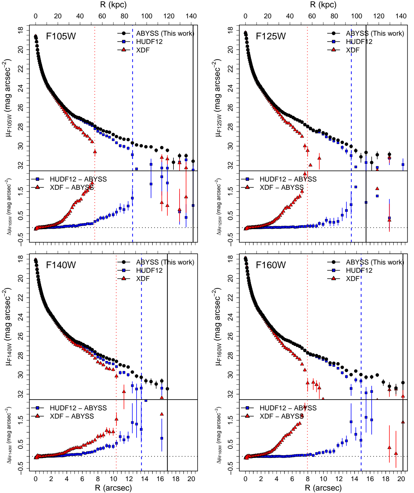
Fig. 20. Comparison of the surface brightness profiles of the elliptical galaxy HUDF-5 ( \alpha = 53.15545 , \delta = -27.79150 , Buitrago et al. 2017) for the F105W (top left panel), F125W (top right panel), F140W (bottom left panel) and F160W filters (bottom right panel), using our own reduction of the HUDF WFC3 mosaics (ABYSS, black dots), the HUDF12 (Koekemoer et al. 2012, blue squares) and the XDF (Illingworth et al. 2013, red triangles). The top plot of each panel shows the surface brightness profile for each reduction. Black solid, blue dashed and red dotted lines represent the elliptic aperture with largest semi-major axis that presents an S/N higher than 3 over the sky-level. The bottom plot represents the difference in magnitude of each previous reduction with the ABYSS version of the mosaics as a function of galactocentric radius. Consult the legend on the figure.
