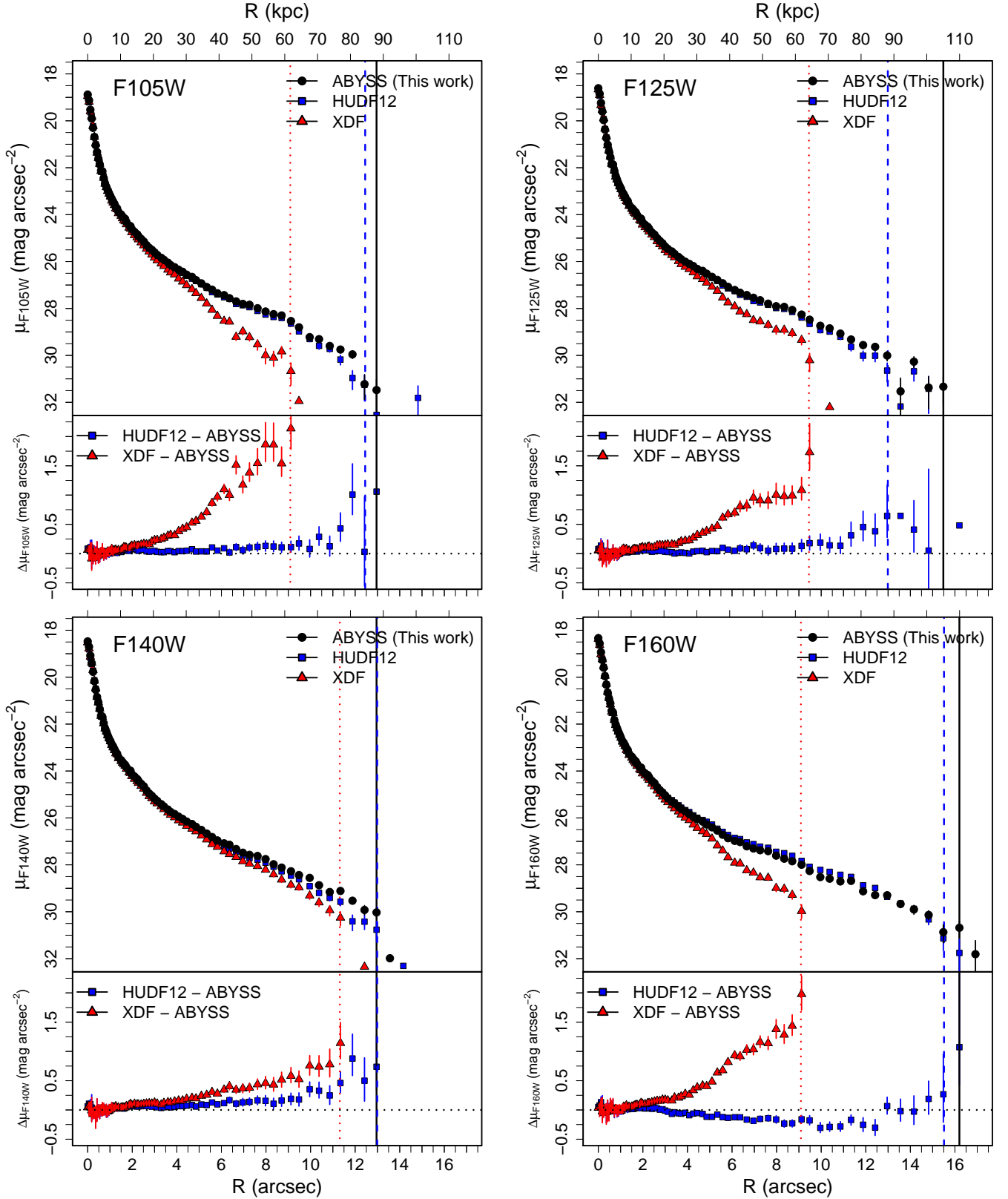
Fig. A.2. Comparison of the surface brightness profiles of the elliptical galaxy HUDF-2 ( \alpha = 53.17254, \delta = -27.78812 , Buitrago et al. 2017 ) for the F105W (top left panel), F125W (top right panel), F140W (bottom left panel), and F160W filters (bottom right panel), using our own reduction of the HUDF WFC3 mosaics (ABYSS, black dots), the HUDF12 ( Koekemoer et al. 2012 , blue squares) and the XDF ( Illingworth et al. 2013 , red triangles). The top plot of each panel shows the surface brightness profile for each reduction. Black solid, blue dashed and red dotted lines represent the elliptic aperture with largest semi-major axis that presents an S/N higher than 3 over the sky-level. The bottom plot represents the difference in magnitude of each previous reduction with the ABYSS version of the mosaics as a function of galactocentric radius. Consult the legend on the figure.
