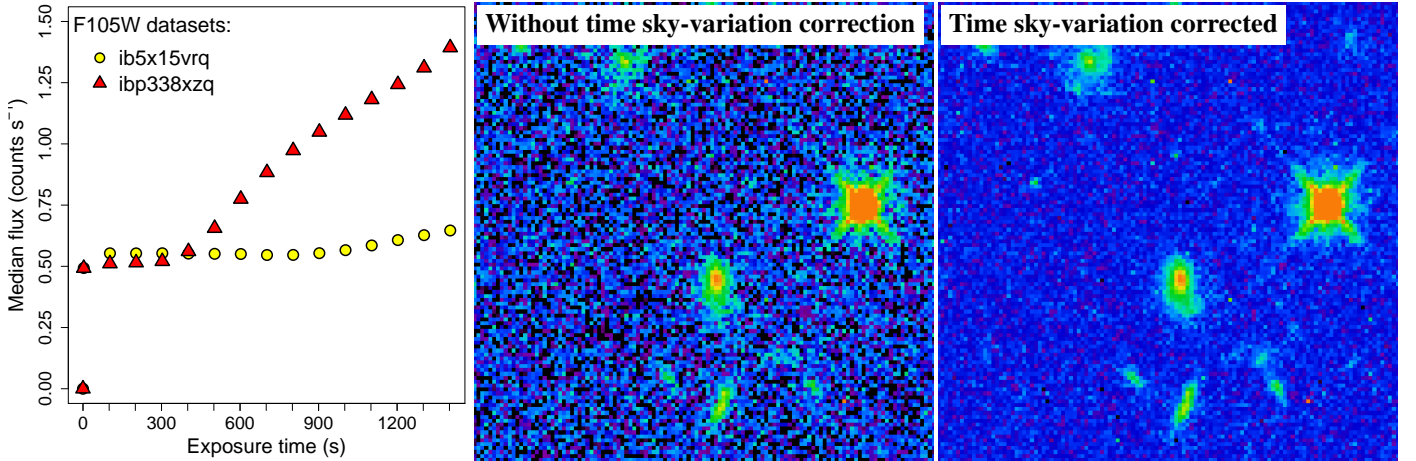
Fig. 7. Example of the effects of time varying sky background in two different datasets of WFC3 IR in the F105W band. Left panel: median background flux of ib5x15vrq (yellow circles) and ibp338xxzq (red triangles). While the dataset ib5x15vrq shows a nearly constant flux on all the different readouts ( \sim 0.50 counts s -1 ), ibp338xxzq is clearly affected by time variation of the sky background, increasing from \sim 0.50 counts s -1 to \sim 1.3 counts s -1 after 400 s from the start of the exposure. Middle panel: sky-corrected ibp338xxzq flt.fits image without time-varying sky background correction applied. Right panel: sky-corrected ibp338xxzq flt.fits image accounting for the time-varying sky background correction. Both images are set to the same colour scale.
