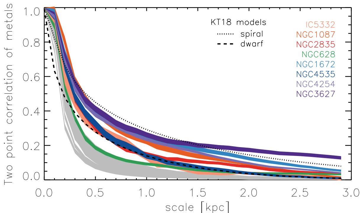
Figure 6. Two-point correlation of metallicity, \Delta(O/H) (after removing the radial gradient) as a function of separation between H II regions, comparing all galaxies. The bands show the 1\sigma distribution given 100 different instances of Gaussian sampling the metallicity uncertainties. The null hypothesis (in grey), that metallicities are uncorrelated, is tested by performing this analysis when all values have been randomized, where the bands show the 1\sigma distribution given 100 different realizations of the shuffling. Most galaxies show correlations at the 30 per cent level out to nearly kpc scales (see also Fig. 7). Black lines are from the KT18 (Krumholz & Ting 2018) model. The dotted and dashed lines represent the fiducial spiral and dwarf galaxies, respectively, to give a sense of how increased star formation and stellar mass impact the model shape. Galaxy names are ordered by stellar mass, from low (orange) to high (purple).
