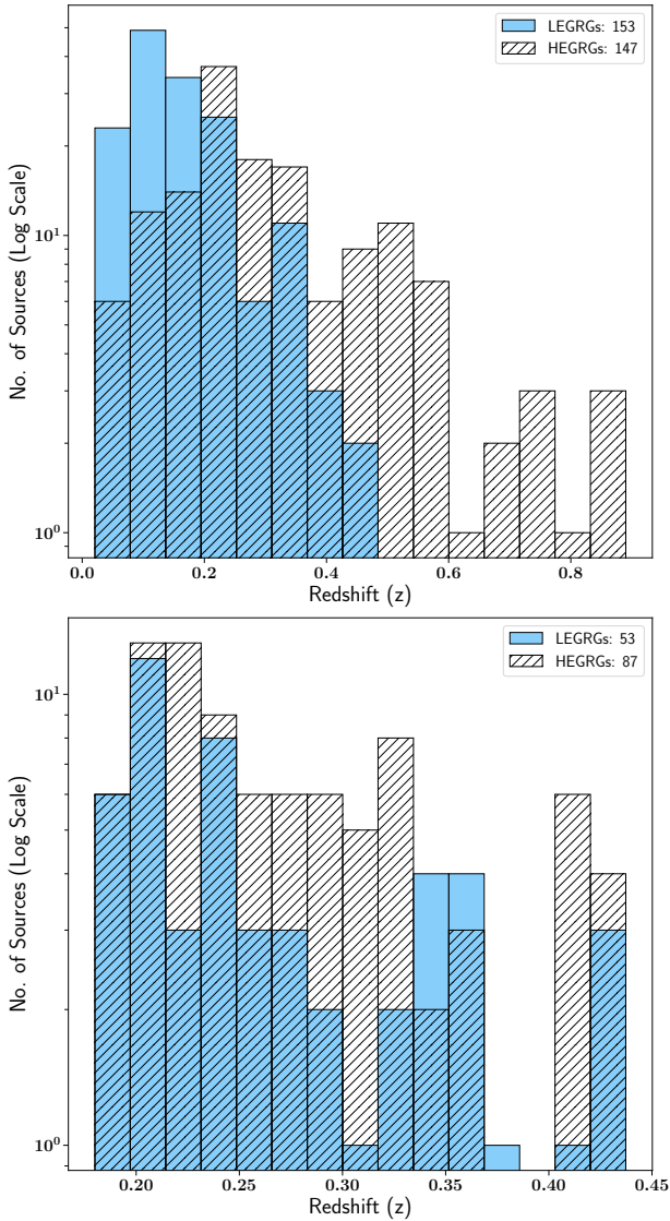
Fig. 8. Redshift ( z ) distributions of LEGRGs and HEGRGs for 0.02 < z < 0.89 (unmatched redshift), represented in not-hatched and hatched bins, respectively in the upper plot. Similarly, in lower plot distributions are shown for matched redshift high- z : 0.18 < z < 0.43 sample of LEGRGs and HEGRGs.
