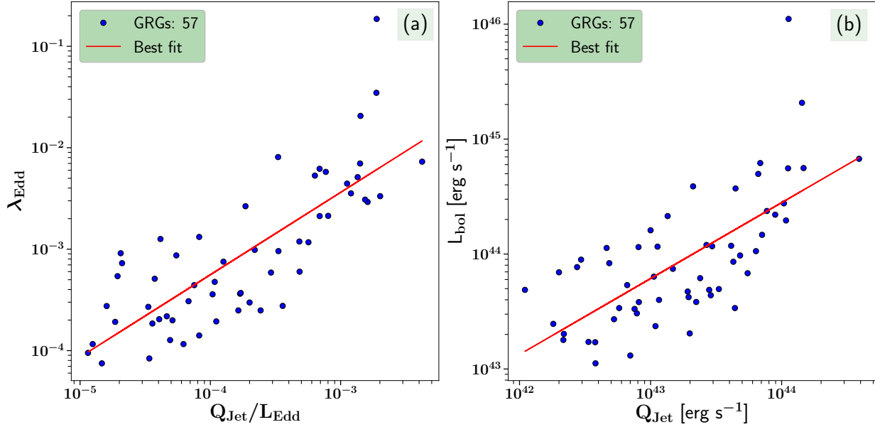
Fig. 13. Panel a : linear correlation for 57 objects between the Eddington ratio ( \lambda_{\text{Edd}} ) and the ratio of the jet kinetic power ( Q_{\text{Jet}} ) to the Eddington luminosity ( L_{\text{Edd}} ), which can be represented as \log \lambda_{\text{Edd}} = 0.81 \times \log(Q_{\text{Jet}}/L_{\text{Edd}}) - 0.005 , as discussed in Sect. 5.4.2. Panel b : bolometric luminosity ( L_{\text{bol}} ) as a function of jet kinetic power ( Q_{\text{Jet}} ), which takes the equation form \log L_{\text{bol}} = 0.66 \times \log(Q_{\text{Jet}}) + 15.38 . The Spearman correlation coefficient is 0.8 and 0.7 for panels a and b , respectively. The red line indicates the best linear fit of the correlations in the log–log plots.
