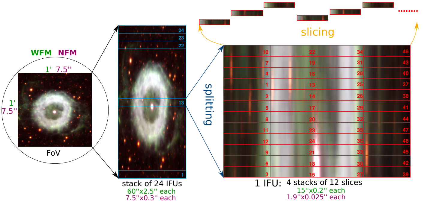
Fig. B.1. Layout of the MUSE instrument, from the focal plane of the VLT (left) to the individual slices (top right). The light from the slices is subsequently dispersed and recorded on the CCD, and there forms the step-pattern visible in Fig. 2. The sizes of the different elements are given as nominal values (green: for WFM, violet: for NFM), the actual sizes are slightly different and change across the field. Overlaid on the images are the channel numbers (on the IFU stack) and the numbers of the slices as counted left to right on the raw data images (on the slicer stack). The example image is a color picture of the planetary nebula NGC 6369, as observed with MUSE in WFM-AO-N on 15 July 2017.
