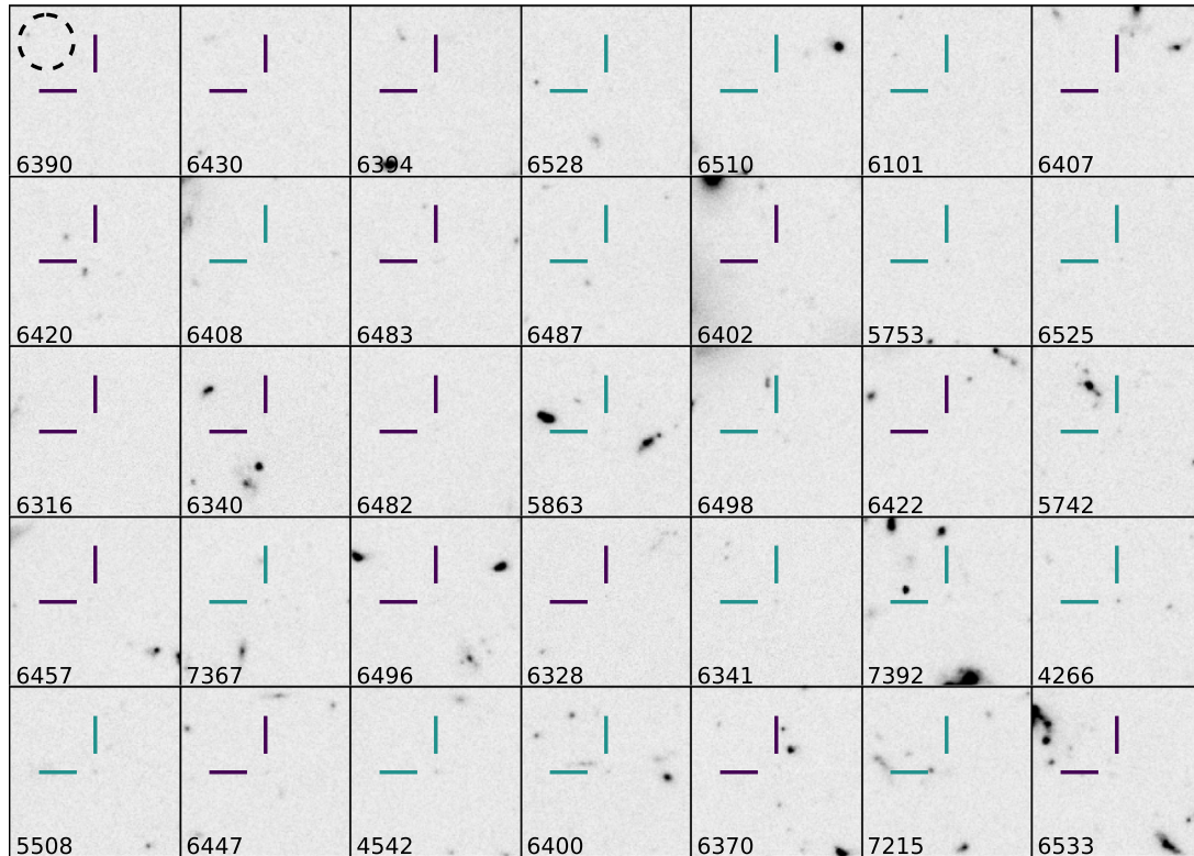
Figure 1. HST/ACS F775W cutouts showing the z \approx 4\text{--}5 LAEs used in this study. Purple cross hairs denote objects that are not detected in any HST photometric band at a significance greater than 3\text{-}\sigma (cf. Maseda et al. 2018), while the blue cross hairs denote an object that is detected only in the HST photometric band that contains Lyman- \alpha emission (i.e. F775W and/or F606W ). Cutouts are 5 arcsec on a side, and the length of the arms of the cross hairs is 1 arcsec. The dashed black circle in the upper-left panel shows the FWHM of the IRAC Ch. 1 PSF (1.6 arcsec diameter). A colour version is available online.
