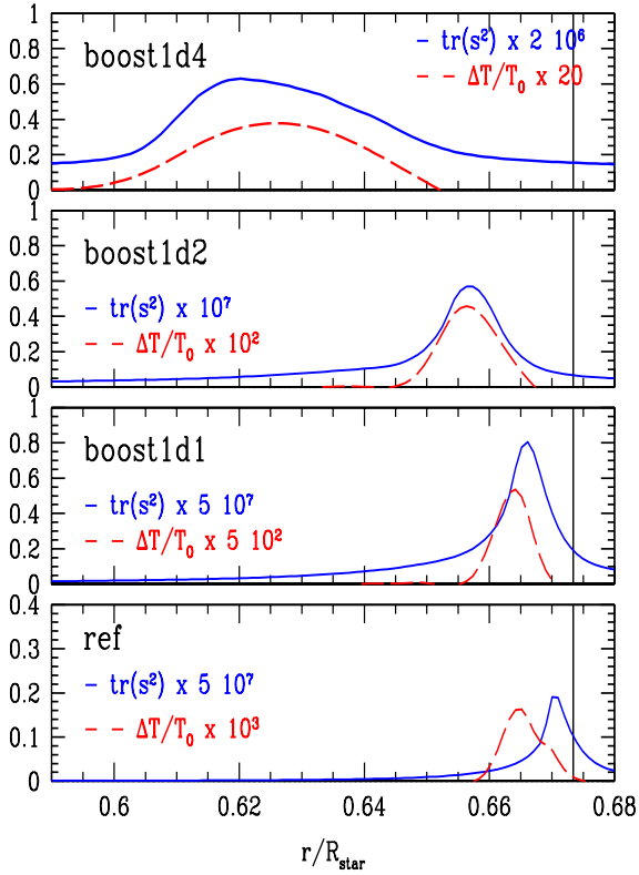
Fig. 7. Radial profile of the time and space averages of the trace of s^2 , \text{tr}(s^2) = s_{r,r}^2 + s_{\theta,\theta}^2 + 2s_{r,\theta}^2 (solid blue lines) in the overshooting layer. The red dashed lines indicate the profile of the relative difference between the time/space average of the temperature \langle\langle T \rangle\rangle_t and the initial profile T_0 . The convective boundary corresponding to the Schwarzschild boundary from the 1D initial model is indicated by the vertical solid line.
