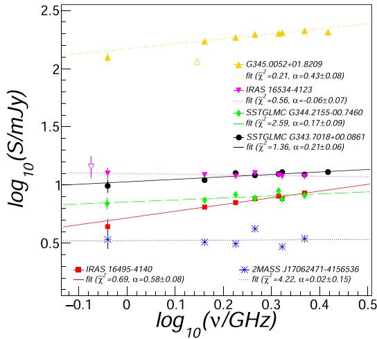
Figure 8. Spectral data of SCORPIO sources associated to stars in the SIMBAD data base, obtained using ASKAP and ATCA data (filled markers) and previous MGPS and NVSS observations (open markers). The power-law fits are reported with coloured lines.
