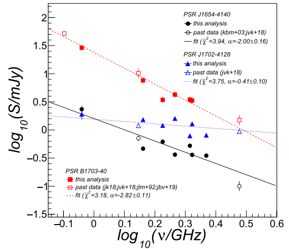
Figure 9. Spectral data for J1654-4140 (open black dots), B1703-40 (open red squares), and J1702-4128 (open blue triangles) pulsars reported in the ATNF pulsar catalogue: kbm + 03 (Kramer et al. 2003), jvk + 18 (Jankowski et al. 2018), jk18 (Johnston & Kerr 2018), jlm + 92 (Johnston et al. 1992), jbv + 19 (Jankowski et al. 2019). ASKAP and ATCA spectral data obtained in this work are shown with filled markers. Single power-law fits are reported with solid, dashed, and dotted lines for the three sample pulsars.
