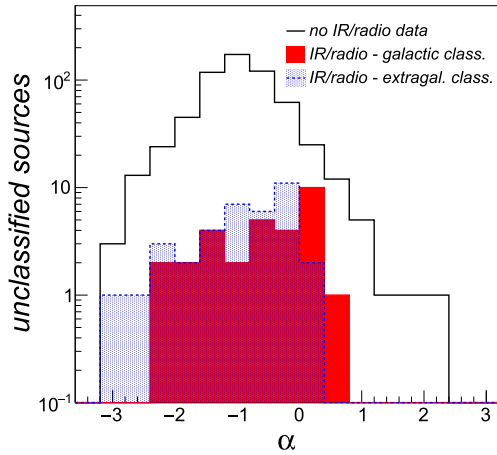
Figure 13. Measured spectral index for unclassified sources. The solid black line histogram includes unclassified sources for which no combined infrared-radio parameter data are available. The filled red and shaded blue histograms include unclassified sources that were classified as Galactic and extragalactic sources, respectively, in the combined infrared-radio analysis.
