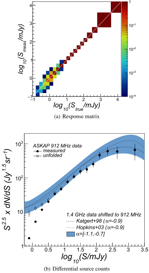
Figure 7. Top: Response matrix used to unfold source detection effects (detection efficiency, flux bias, and uncertainty) from raw source counts. The colour represents the probability r_{ji} for a source with true flux density in bin i to be detected with measured flux density in bin j ; Bottom: Differential uncorrected source counts of the SCORPIO survey catalogue normalized to standard Euclidean counts ( \propto S^{-2.5} ) shown with filled black dots. The open black dots represents the unfolded differential source counts obtained with the procedure described in the text and using the response matrix above. The shaded area represents the existing extragalactic source count data at 1.4 GHz, parametrized by Katgert (1988), Hopkins et al. (2003) and shifted to a frequency of 912 MHz assuming a spectral index \alpha ranging from -1.1 to -0.7 (central value -0.9 ). Values relative to the median spectral index -0.9 are shown as dashed and dotted lines, respectively.
