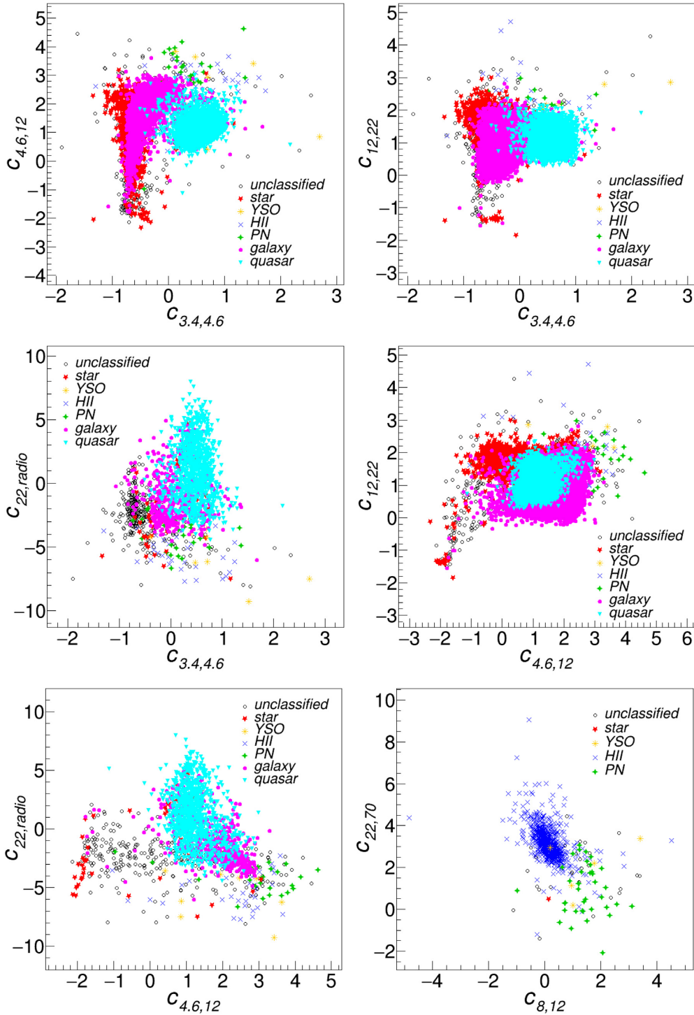
Figure 12. Scatter plots of selected infrared-infrared or infrared-radio colours for different infrared bands (3.4, 4.6, 12, 22, 70 \mu\text{m} ). Unclassified objects are shown with grey smaller dots while pre-classified sources with coloured markers (HII regions: blue crosses, PNe: green diamonds; stars: red stars; YSOs: orange asterisks; galaxies: purple dots, QSO: cyan triangles).
