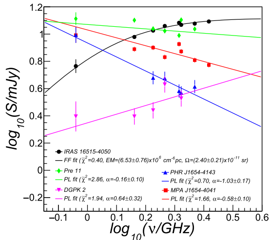
Figure 10. Radio continuum spectra for five PNe obtained using ASKAP and ATCA observations.
