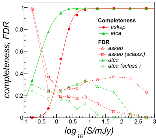
Figure 3. Completeness (filled markers) and false detection rate (FDR) (open markers) as a function of the injected and measured source flux density, respectively, obtained on the simulated ASKAP (red markers) and ATCA (green markers) source catalogues. The solid lines represent the fitted completeness model of equation (1). The open squares and diamonds (labelled as ‘sclass’) represent the false detection rate obtained after applying a neural network classifier, trained to identify spurious fit components in the catalogue.
