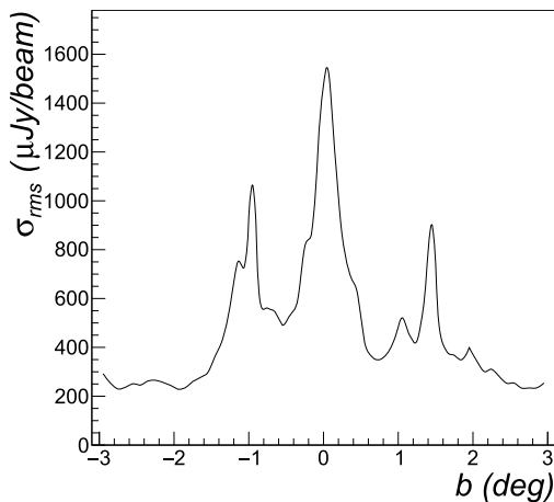
Figure 2. Estimated background noise of SCORPIO mosaic in \mu\text{Jy beam}^{-1} as a function of the Galactic latitude b and averaged over Galactic longitude l .
