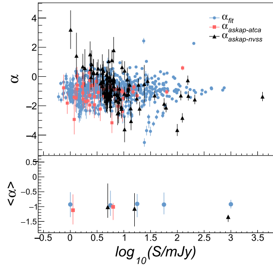
Figure 6. Top panel: Spectral indices of ASKAP 912 MHz source components as a function of ASKAP flux density. The blue dots represent the spectral indices obtained from a power-law fit of available ASKAP–ATCA–NVSS–MGPS data, while the red squares and black triangles indicate the spectral indices obtained from only ASKAP–ATCA and ASKAP–NVSS frequencies, respectively. Bottom panel: Median spectral index for the three samples as a function of ASKAP flux density. Error bars are the interquartile range (IQR) in each flux density bin.
