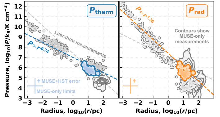
Fig. 6. Thermal ( left panel ) and direct radiation ( right panel ) pressure terms. Coloured points are H II regions studied in this work, grey points are measurements from the literature (Lopez et al. 2014; McLeod et al. 2019, 2020, 2021; Barnes et al. 2020; Olivier et al. 2021), and the contours show the upper and lower limits for all galaxies studied by Barnes et al. (2021). The dashed lines show the power law relations from Olivier et al. (2021).
