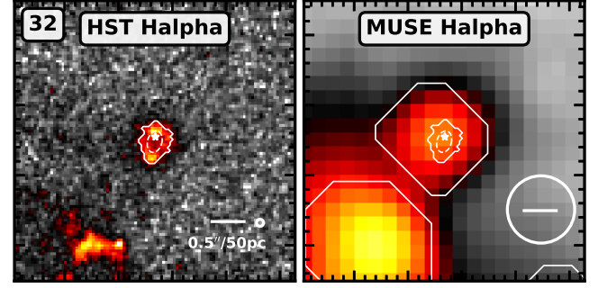
Fig. 2. Comparison between the HST and MUSE observations towards one of the H II regions in our sample. HST \text{H}\alpha narrowband emission overlaid with a contour outlining the isophotal boundary as defined from our dendrogram analysis, shown on the left. We show the intensity-weighted second order moment of the structure within this boundary as a dashed ellipse, which we use to define the radius of the H II region (Sect. 3.1). A star marks the position of the identified ionising stellar population (Sect. 3.2). The region ID is shown in the upper left (Table A.1). \text{H}\alpha emission observed with MUSE ( Emsellem et al. 2022 ), overlaid with white contours showing the boundaries of sources identified as part of the nebula catalogue from Santoro et al. (2022) , shown on the right. In the lower right of each panel, we show a scale bar and a circle denoting the approximate PSF size.
