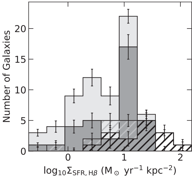
Figure 12. The same as Figure 6 but for \Sigma_{\text{SFR}} derived from H \beta .
