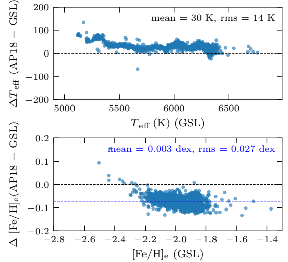
Fig. 5. Comparison between T_{\text{eff}} and [\text{Fe}/\text{H}]_e obtained with GSL and AP18 grids. Top panel: difference between T_{\text{eff}} ( \Delta T_{\text{eff}}(\text{AP18} - \text{GSL}) ), computed by subtracting the GSL results from the AP18 results) as a function of T_{\text{eff}} values with GSL. Bottom panel: difference of equivalent iron abundance ( \Delta[\text{Fe}/\text{H}]_e ) as a function of the iron abundance with GSL. The dashed blue line shows the expected bias due to the different level of \alpha -element enhancement in the two grids (0.4 vs. 0.5 dex, see the text for details). In both panels we report the mean and rms of the differences.
