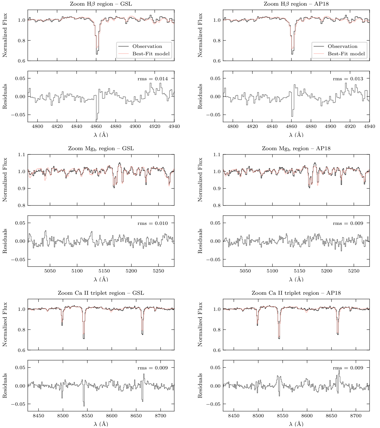
Fig. 2. Typical fits of a spectrum (ID=id0000010747jd2456866p4985f000). The fit, performed over the complete wavelength range, 4750–9300 Å, returned T_{\text{eff}} = 5471 K and [\text{Fe}/\text{H}]_{\text{e}} = -1.84 dex for global rms residuals of 0.01 for both GSL and AP18. The left column shows the [\alpha/\text{Fe}] = 0.4 dex GSL grid, and the right column presents the [\alpha/\text{Fe}] = 0.5 dex fine AP18 grid. The top row shows a small wavelength region around the \text{H}\beta line, the middle row shows a region around the \text{Mg}_b triplet, and the bottom one shows a region around the Ca II triplet. For each plot, the top panel presents the observation (black line) with the best-fit model over-plotted in red. The bottom panel presents the residuals, observation minus model.
