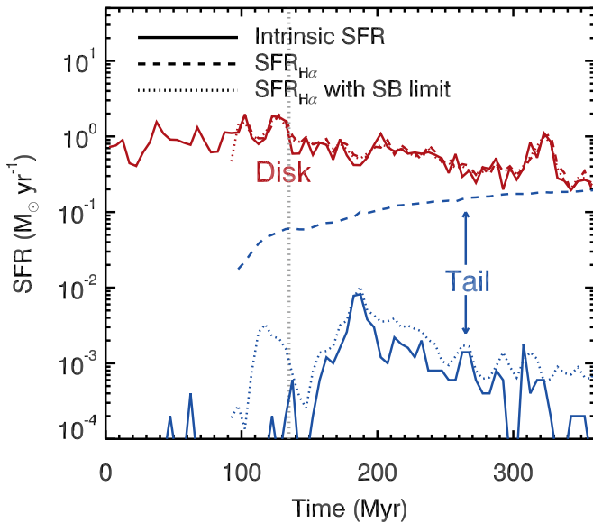
Figure 12. Evolution of the intrinsic SFR (solid) and the SFR estimated from the total unobscured H \alpha luminosity (SFR _{\text{H}\alpha} ; dashed and dotted). The red and blue colors indicate the SFRs in the disk and tail, respectively. We present SFR _{\text{H}\alpha} with (dotted) and without (dashed) an SB limit of 6 \times 10^{38} \text{ erg s}^{-1} \text{ kpc}^{-2} . We display the SFR _{\text{H}\alpha} lines only at t > 100 Myr. The vertical dotted line marks the epoch at which the wind front reaches the galaxy. SFR _{\text{H}\alpha} closely traces the intrinsic SFR in the disk, while the majority of the H \alpha SB (dashed) in the tail originates from processes other than star formation. However, the intrinsic SFR in the tail is reasonably recovered by considering H \alpha bright regions (dotted).
