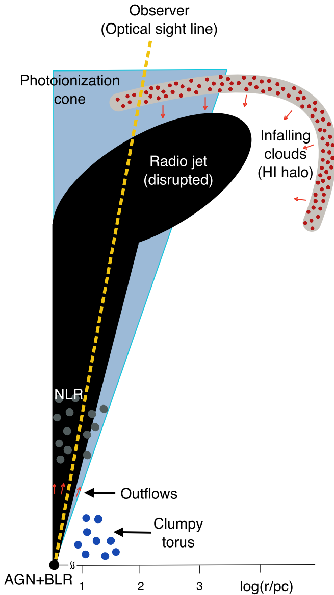
Figure 3. Cartoon depicting a quadrant of M1540–1453 embedded in a clumpy ISM. The quasar’s optical sight line (dashed line) may not intercept infalling high- N(\text{H I}) clouds. In comparison, extended radio emission ( >425 pc) from the lobes will be intercepted by several such clouds, producing the broad redshifted H I 21 cm absorption line. The extent of the H I halo and radio emission could be as large as 10 kpc.
