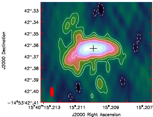
Figure 2. The VLBA 1.53 GHz image of M1540–1453. The rms noise in the image is 65 \mu\text{Jy beam}^{-1} . The restoring beam of 9.0 \text{ mas} \times 3.1 \text{ mas} with a position angle of +2^\circ 4' is shown as an ellipse at the bottom left corner. The contour levels are 250 \times (-2, -1, 1, 2, 4, 8, 16, \dots) \mu\text{Jy beam}^{-1} . The peak intensity is 6.3 \text{ mJy beam}^{-1} . The plus sign represents the location of the putative radio core/AGN.
