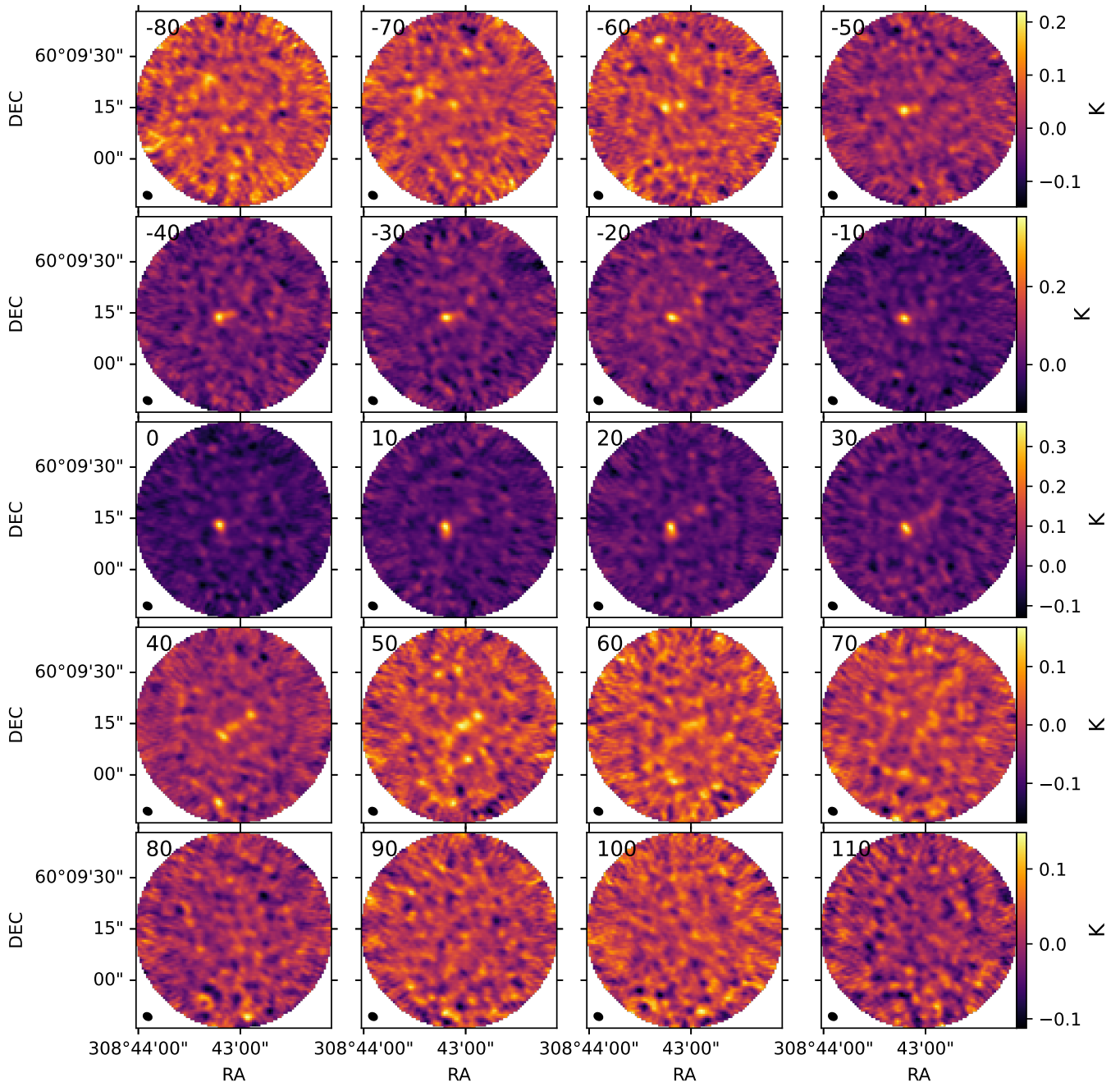
Fig. A.8. N_2H^+ channel maps, from -80 to 110 \text{km s}^{-1} .
