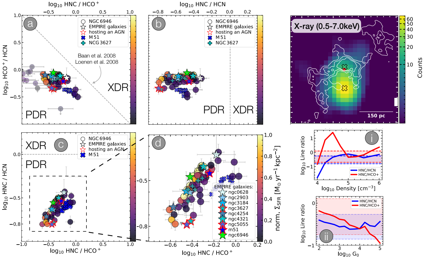
Fig. 8. Diagnostic plots using integrated line ratios of HCN, HNC and \text{HCO}^+ versus each other. Left panels: (a): integrated \text{HCO}^+/\text{HCN} versus \text{HNC}/\text{HCO}^+ ratios. (b): integrated \text{HCO}^+/\text{HCN} versus \text{HNC}/\text{HCN} ratios. (c): integrated \text{HNC}/\text{HCN} versus \text{HNC}/\text{HCO}^+ ratios. The grey dashed lines mark the boarder between XDR and PDR (Baan et al. 2008; Loenen et al. 2008). Circles indicate reliable values ( S/N > 5 ) and upper limits for the central 20'' \approx 745 pc towards NGC 6946. Stars show the EMPIRE galaxies and stars with red contours present galaxy centres hosting an AGN (Goulding & Alexander 2009). For two of them we find ancillary data: the cross shaped markers show the \sim 4'' ( \approx 166 pc) M 51 observations (Querejeta et al. 2016) and the \sim 2'' ( \approx 100 pc) NGC 3627 observations (Bešlić et al. 2021). (d): the enclosed integrated \text{HNC}/\text{HCN} versus \text{HNC}/\text{HCO}^+ with the kpc-sized centres of the EMPIRE survey (see Jiménez-Donaire et al. 2019 for details). NGC 6946 and the EMPIRE galaxies are in the PDR regime in all panels. Interestingly, EMPIRE galaxies harbouring an AGN do not show an enhancement of HCN as suggested in many studies (see text for a discussion). We run (Meijerink & Spaans 2005) PDR models for the observed ranges of line ratios (blue and red shaded areas) by (i) fixing the radiation field and (ii) fixing the density. The red and blue lines show the model output (more in text). The colours in (a–d) indicate \Sigma_{\text{SFR}} . We have normalised them to the mean \Sigma_{\text{SFR}} value and find no trend with the integrated line ratios. Upper right panel: X-ray 0.5–7.0 keV in counts for NGC 6946 with integrated CO(2–1) contours on top. The black crosses mark the positions of the detected X-ray sources by Holt et al. (2003) which are not strong enough to trigger a XDR.
