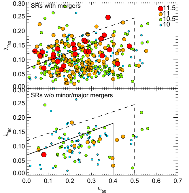
Figure 5. \lambda_{r50} as a function of \epsilon_{r50} at z = 0 for SRs in EAGLE. The top panel shows SRs that have had mergers with mass ratios \geq 0.1 in the last 10 Gyr, while the bottom panel shows the complement SRs. Sizes and colours of the symbols correspond to different stellar masses, as labelled in the top panel. For reference we show as solid and dashed lines the parametric classifications of Cappellari (2016) and van de Sande et al. (2021), respectively.
