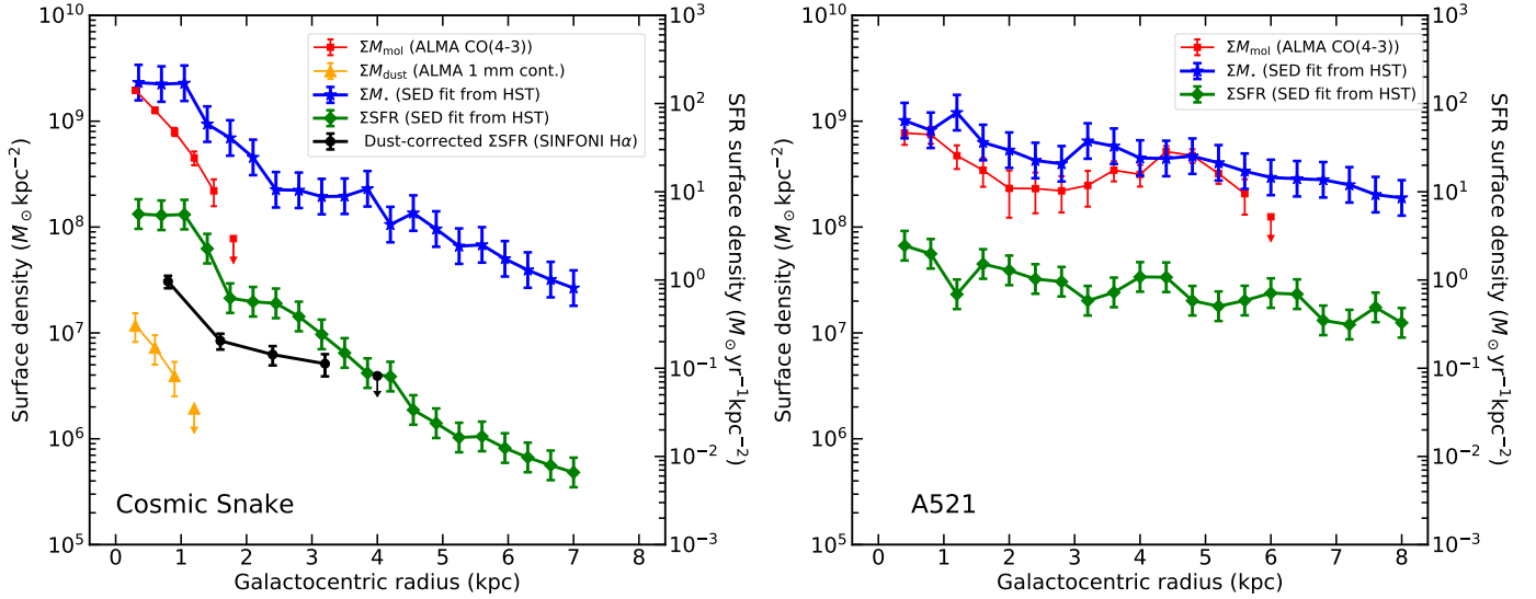
Fig. 7. Radial profiles of the Cosmic Snake ( left panel ) and A521 ( right panel ). The blue lines trace the \Sigma M_* profile, the red and orange lines trace the \Sigma M_{\text{mol}} and \Sigma M_{\text{dust}} profiles, and the green and black lines trace the \Sigma \text{SFR} radial profiles from the SED fits and the H \alpha emission, respectively. We consider as detection a signal above 4\sigma for the ALMA data and above 2\sigma for the other data. We indicate with an upper limit the datapoint below the corresponding detection threshold.
