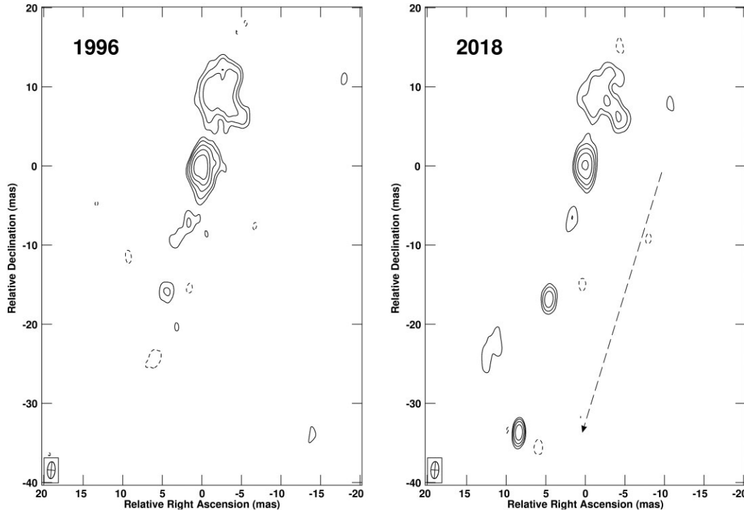
Figure 4. X-band VLBA images of CTA 21 from 1996 January 3 and 1996 March 13 (combined; experiment BB023, Beasley et al. 2002, left) and from 2018 November 3 (experiment UG002S, right). The southernmost bright compact component that appears in 2018 was not detected in 1996. The arrow represents the amount and direction of the positional displacement between the two epochs as observed in the astrometric programmes (Fig. 3). The lowest contours are at \pm 5 mJy beam ^{-1} in both images, the positive levels increase by a factor of 2. The half-power beamwidth is indicated in the lower-left corner. The peak brightnesses are 156 mJy beam ^{-1} (1996) and 91 mJy beam ^{-1} (2018). The calibrated data sets were obtained from the Astrogate data base, and the images made in Difmap (Shepherd 1997) and plotted in AIPS (Greisen 2003).
