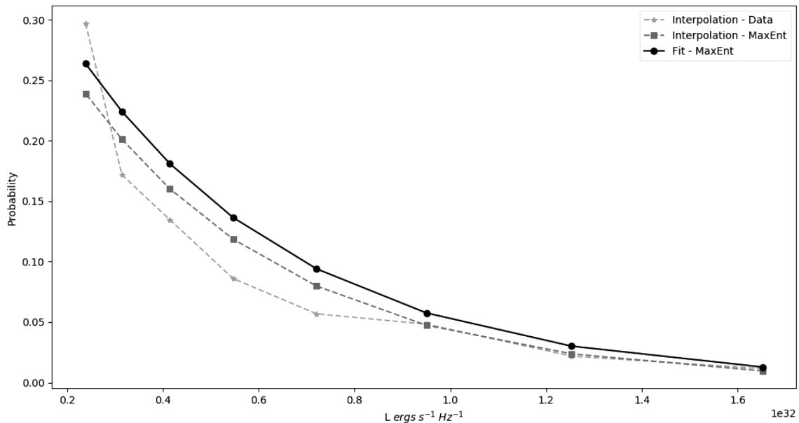
Figure 3. Luminosity function obtained from MaxEnt using the fitting curve to z = 3.5 .
