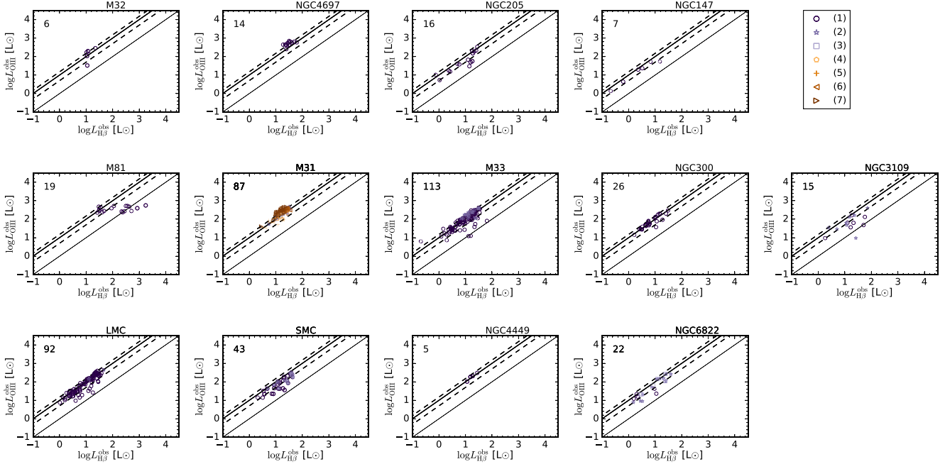
Figure 16. Values of \log L_{\text{[O III]}}^{\text{obs}} as a function of \log L_{\text{H}\beta}^{\text{obs}} . Upper panels: early-type galaxies, middle panels: spiral galaxies, lower panels: irregular galaxies. The number that appears at the top left corner of each panel indicates the number of PNe plotted in each panel. The thin line represents where L_{\text{[O III]}}^{\text{obs}} = L_{\text{H}\beta}^{\text{obs}} , the thick solid line and the dashed lines are obtained from the mean and the standard deviation of L_{\text{[O III]}}^{\text{obs}}/L_{\text{H}\beta}^{\text{obs}} . The numbering of the references is the same as in Fig. 3.
