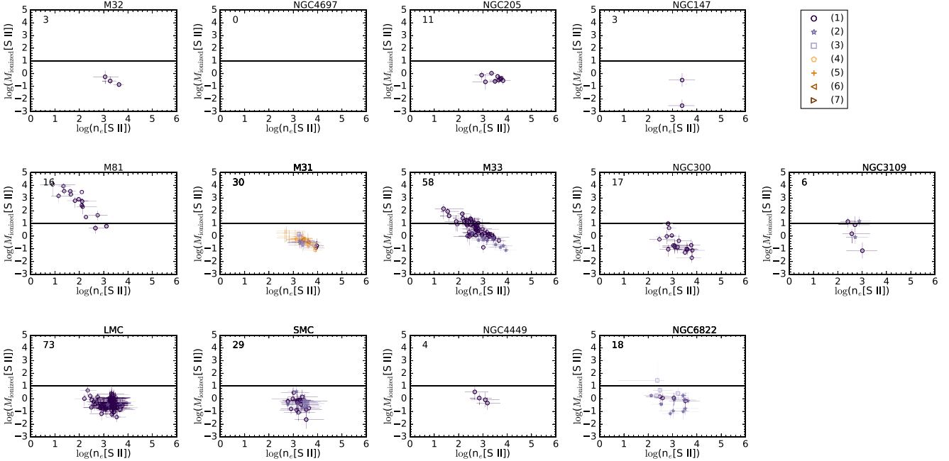
Figure 7. Values of the ionized mass as a function of the electron density derived both from [S II] lines. Upper panels: early-type galaxies, middle panels: spiral galaxies, lower panels: irregular galaxies. The number that appears at the top left corner of each panel indicates the number of PNe plotted in each panel. The numbering of the references is the same as in Fig. 3.
