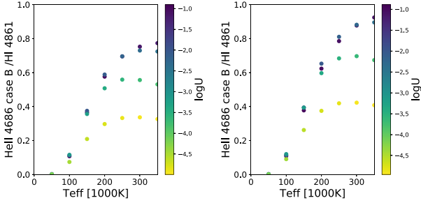
Figure A1. Values of \text{He II}/\text{H}\beta as a function of the effective temperature for a sample of photoionization models. Left-hand panel: \text{He}/\text{H} = 0.10 , right-hand panel \text{He}/\text{H} = 0.15 . The colour bar runs from low to high ionization parameter values.
