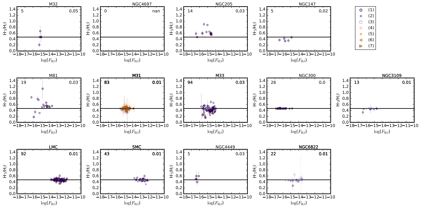
Figure 5. Assessment of accuracies in line fluxes. Values of H\gamma/H\beta as a function of F_{H\beta} . Upper panels: early-type galaxies, middle panels: spiral galaxies, lower panels: irregular galaxies. The number that appears at the top left corner of each panel indicates the number of PNe plotted in the panel. The number that appears at the top right corner of each panel indicates the weighted standard deviation of the H\gamma/H\beta values divided by its theoretical value. The numbering of the references is the same as in Fig. 3.
