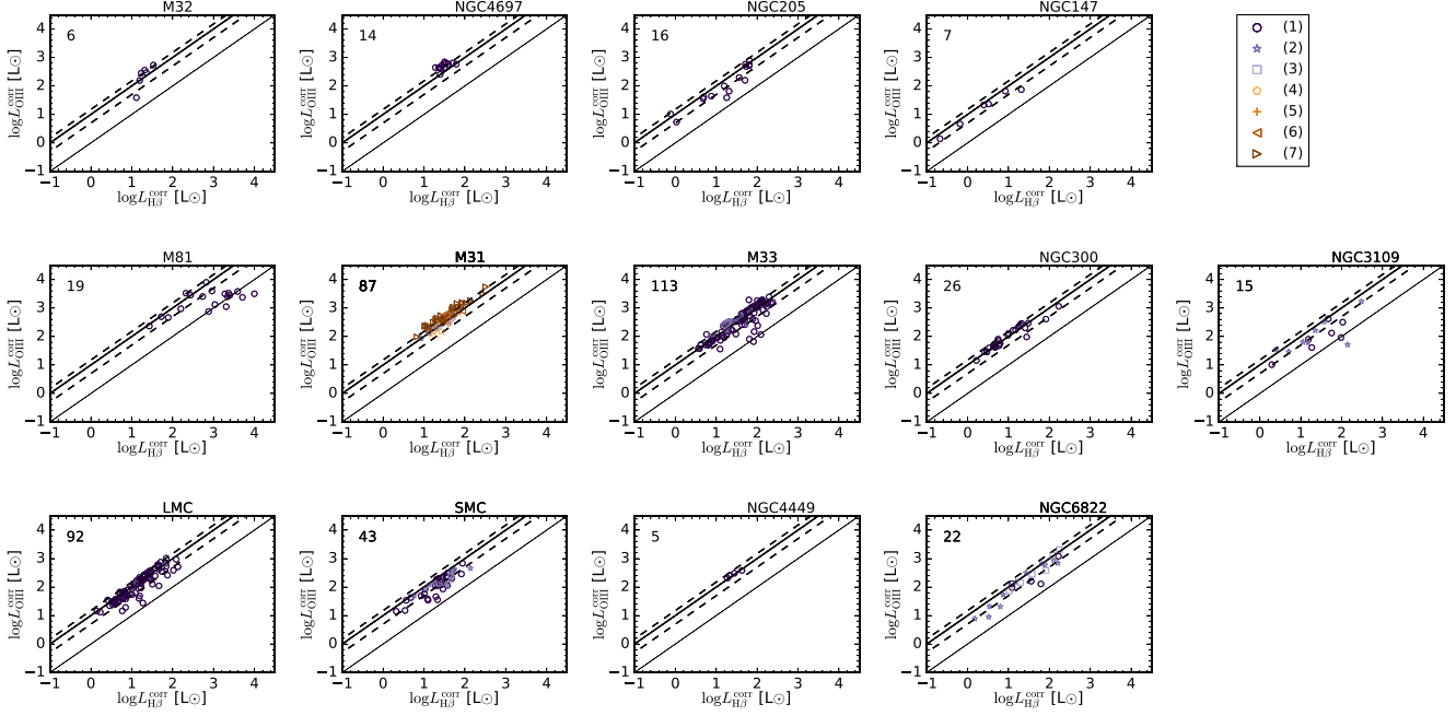
Figure 15. Values of \log L_{\text{[O III]}}^{\text{corr}} as a function of \log L_{\text{H}\beta}^{\text{corr}} . Upper panels: early-type galaxies, middle panels: spiral galaxies, lower panels: irregular galaxies. The number that appears at the top left corner of each panel indicates the number of PNe plotted in each panel. The thin line represents where L_{\text{[O III]}}^{\text{corr}} = L_{\text{H}\beta}^{\text{corr}} , whereas the thick solid line and the dashed lines are obtained from the mean and the standard deviation of L_{\text{[O III]}}^{\text{corr}}/L_{\text{H}\beta}^{\text{corr}} . The numbering of the references is the same as in Fig. 3.
