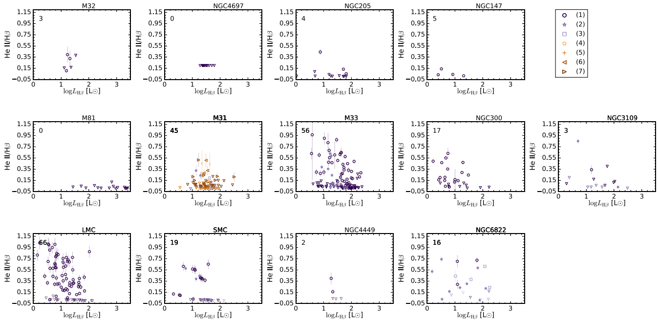
Figure 13. Values of \text{He II } \lambda 4686/H\beta as a function of \log L_{H\beta} . Upper panels: early-type galaxies, middle panels: spiral galaxies, lower panels: irregular galaxies. The number that appears at the top left corner of each panel indicates the number of PNe plotted in each panel. The numbering of the references is the same as in Fig. 3.
