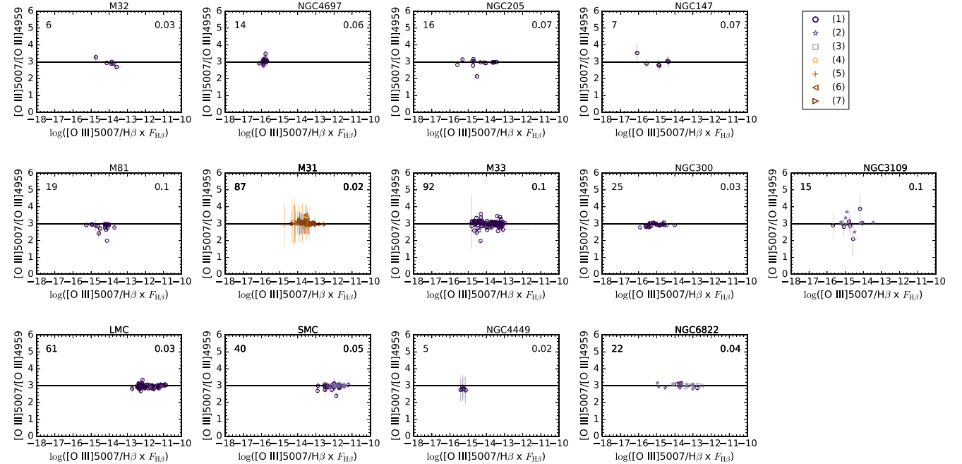
Figure 4. Assessment of accuracies in line fluxes. Values of [O III] \lambda 5007/\lambda 4949 ratio as a function of [O III] \lambda 5007/H\beta \times F_{H\beta} . Upper panels: early-type galaxies, middle panels: spiral galaxies, lower panels: irregular galaxies. The number that appears at the top left corner of each panel indicates the number of PNe plotted in the panel. The number that appears at the top right corner of each panel indicates the weighted standard deviation of the [O III] \lambda 5007/\lambda 4949 values divided by its theoretical value. The numbering of the references is the same as in Fig. 3.
