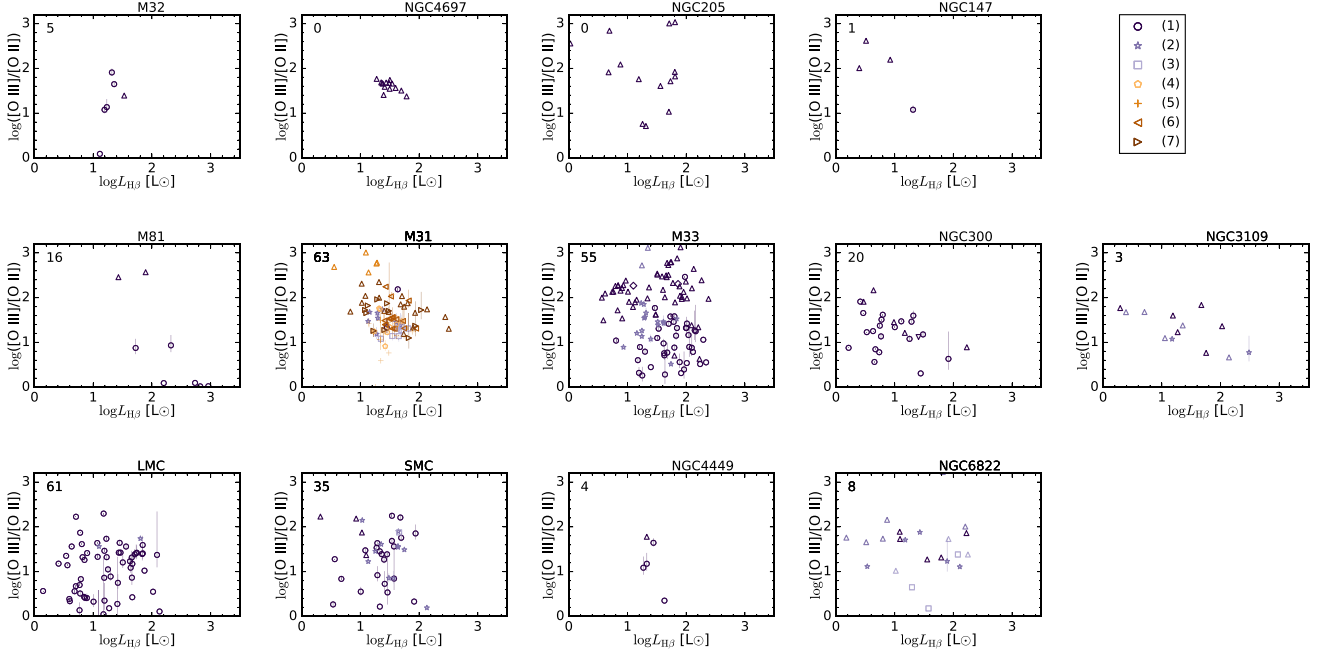
Figure 14. Values of \log([\text{O III}] \lambda 5007/[\text{O II}] \lambda 3727) as a function of \log L_{\text{H}\beta} . Upper panels: early-type galaxies, middle panels: spiral galaxies, lower panels: irregular galaxies. The number that appears at the top left corner of each panel indicates the number of PNe plotted in each panel. The numbering of the references is the same as in Fig. 3.
