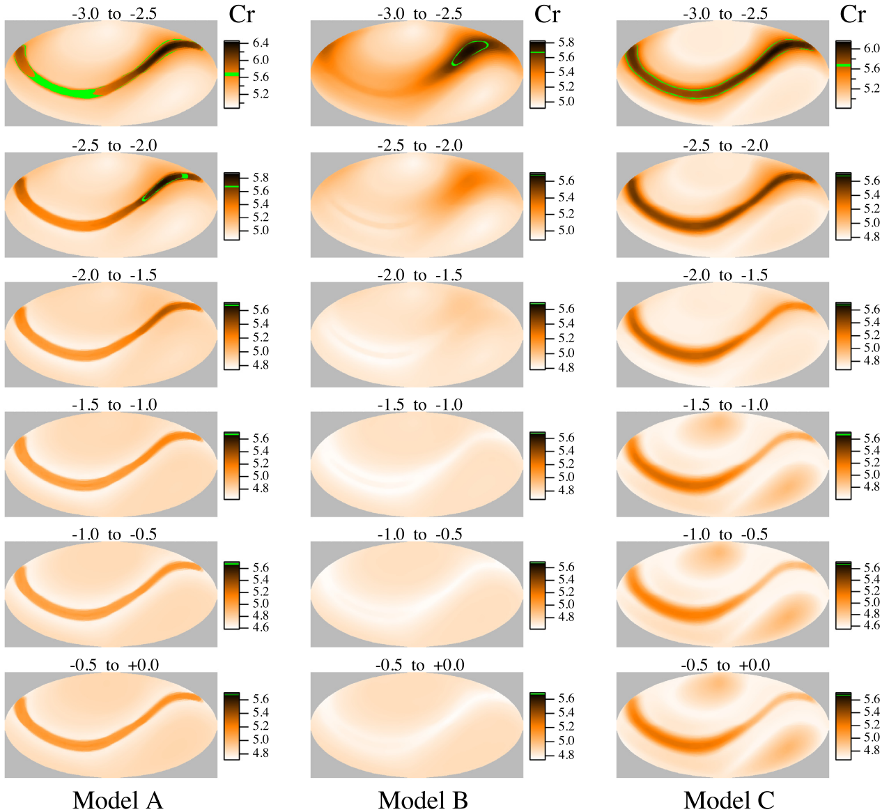
Figure 5. Same as Fig. 4, for Cr. The green colour marks positions where the Cr abundance is solar ( 5.67 \pm 5 per cent). Note that Cr is underabundant in all slabs with \log \tau \gtrsim -2.0 .
