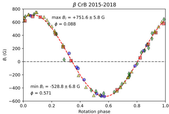
Figure 4. The figure shows the rotational modulation of B_l for \beta CrB from 73 observations corresponding to magnetic maps from 2015 to 2018. The data from 2015 are shown as blue circle, 2016 red square, 2017 yellow triangle, and 2018 green diamond. The dashed red curve indicates a fitted sine curve to the data with a period of 18.4868 d that corresponds to the rotation period used in ZDI analysis. The rotation phase \phi corresponds to the measured maximum and minimum B_l . The figure shows the magnetic field is stable over the 4 yr observation period. The zero day is the first date of B_l measurement on 2018 January 23.
