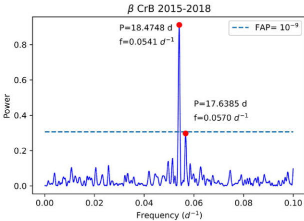
Figure 3. Figure at left: GLS periodogram a time-series of B_l measurements for \beta CrB spanning 1240 d from 2015 March 7 to 2018 July 28 (Table 1). The figure shows the power versus frequency and FAP, with the highest peaks marked with a red circle, and text describing the associated period and frequency. The FAP quantifies the probability of the maximum peak being produced by a signal without a periodic component. The blue dashed line is FAP 10^{-9} level, which indicates an excellent detection for the period determination. The best sine period determined from the GLS periodogram is 18.4748 \pm 0.005 d. The figure at top right shows the time spacing of the observations. Figure at bottom right shows the window function.
