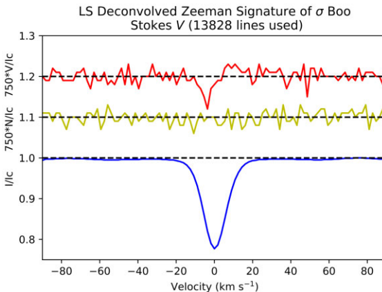
Figure 2. Mean LSD profile for \sigma Boo on 2021 May 18. The upper line (red) shows the Stokes V profile (y-axis expanded by 750 times and shifted up by 0.2 to allow better visibility). The middle line (green-yellow) shows the null profile (expanded by 750 times and shifted up by 0.1), which is used as a check for any spurious signals contaminating the spectra. The lower line (blue) shows the Stokes I profile.
