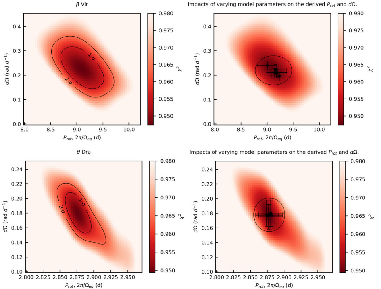
Figure 5. Figures at left: Surface differential rotation contour plot for \beta Vir 2017 April 3–24 (top) and \theta Dra 6–2017 April 24 (bottom) with 1\sigma , and 2\sigma confidence contours marked with black lines. From the \chi^2 landscape we determine the rotation period at the 1\sigma level of \beta Vir as 9.1 \pm 0.4 d and \theta Dra 2.88 \pm 0.02 . The d\Omega for \beta Vir is 0.23 \pm 0.09 rad d ^{-1} and \theta Dra 0.18 \pm 0.03 rad d ^{-1} . Figures at right: Surface differential rotation using \chi^2 minimization landscape of Stokes V profiles for \beta Vir (top) and \theta Dra (bottom). The variation ellipse is generated by individually varying stellar parameters and determining the corresponding \Omega_{\text{eq}} and d\Omega pairs. The parameters varied for \beta Vir are v \sin i ( \pm 2.6 km s ^{-1} ), inclination angle ( \pm 2 deg), and \chi^2 aim ( \pm 0.05 ), for \theta Dra v \sin i ( \pm 0.2 km s ^{-1} ), inclination angle ( \pm 2 deg), and \chi^2 aim ( \pm 0.05 ). The individual error bars indicate the 1\sigma errors of a Gaussian fit to the \chi^2 landscape.
