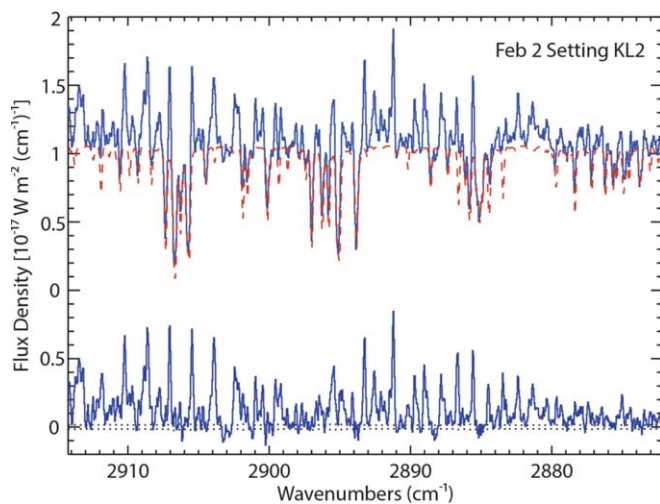
Figure 1. Flux-calibrated, high-resolution ( \lambda/\Delta\lambda \sim 25,000 ) spectral extracts and residuals in C/2014 Q2 (Lovejoy) in setting KL2 order 22. The spectrum is co-added over a 3 spectral \times 9 spatial pixel extract ( 0''.432 \times 1''.71 ) centered on the peak of the gas emission. The solid blue trace at the top of the panel is the comet spectrum with the best-fit synthetic atmospheric model superimposed (dashed red trace). Molecular lines from the comet are seen as emissions in the comet spectrum above the atmospheric model. The solid blue trace at the bottom of the panel is the continuum-subtracted spectral residuals. The dotted black curves superimposed on the comet residuals represent the estimated \pm 1\sigma channel-by-channel photon noise envelope.
