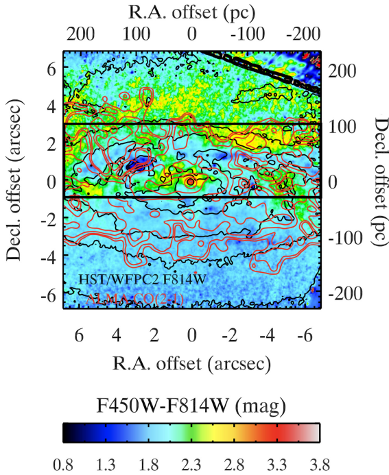
Figure 10. HST WFPC2 F450W – F814W colour map of the nucleus of NGC 3593 (see also Panel A of Fig. B5 in Appendix B), overlaid with ^{12}\text{CO}(2-1) (red) and F814W (black) iso-intensity contours. The black rectangle indicates the region with co-spatial molecular gas and dust extinction discussed in the text.
