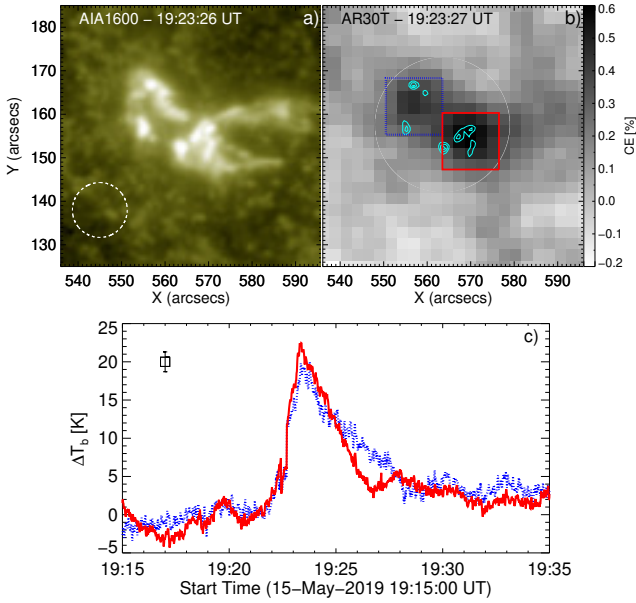
Fig. 6. Close view of the mid-IR and UV sources. Panel a shows the flaring region observed by AIA1600. The dashed white circle indicates the size of the Airy disk of the AR30T. Panel b displays the two bright kernels observed in 30 THz after pre-event subtraction with colors inverted (black is more intense). The dotted-blue and red boxes enclose the northern and southern kernels respectively. The contour levels are 50, 70, and 90% of the flare maximum in AIA1600. The white circle indicates the area used to estimate the mid-IR temporal evolution displayed in Fig. 5. The excess brightness temperature averaged for the boxes shown in the upper panel (with the respective blue and red color) is shown in panel c . The error bar indicates 1\sigma uncertainty in \Delta T_b .
