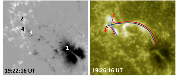
Fig. 8. Close up view of the photospheric magnetic field configuration. Left panel: SDO/HMI line-of-sight magnetogram of AR 12741 on 15 May 2019 at around flare maximum. The numbers indicate the polarities where the loops associated with the energy release during the flare could be anchored. Right panel: AIA1600 image including a sketch of the connectivities related to the loops involved in the flare. Blue and light blue continuous lines indicate loops before reconnection, while red lines would correspond to reconnected loops. Plus and minus signs mark the polarity sign of the footpoints. Both panels cover the same field of view; their sizes are 94'' in the horizontal and 87'' in the vertical directions. The convention for the magnetic field map is the same as in Fig. 2.
