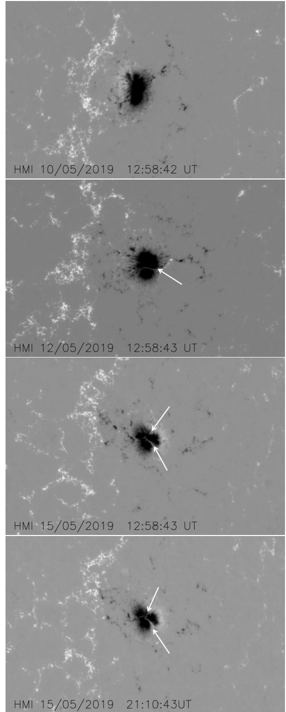
Fig. 1. SDO/HMI line-of-sight magnetograms of AR 12741, with 720 s time resolution, as it traverses the solar disk. The AR is formed by a compact and elongated negative polarity followed by a very dispersed positive field. An east-west light bridge (see white arrow) is clearly observed on the second panel dividing the preceding spot into two sections. MMFs, formed by small bipolar fragments, are seen moving towards the moat region surrounding the spot. The AR is continuously decaying; by 15 May other light bridges are observed (as shown in the third and fourth panels marked by white arrows). The last two panels correspond to the flare day, in the early morning and at night. Black corresponds to negative magnetic field (pointing away from the observer) and white to positive field (towards the observer), the values of the field have been saturated above (below) 1000 G (–1000 G). The images are centered in the main negative polarity with horizontal and vertical sizes of 300'' and 190'', respectively. The online movie HMI-8-17May.mp4 complements this figure.
