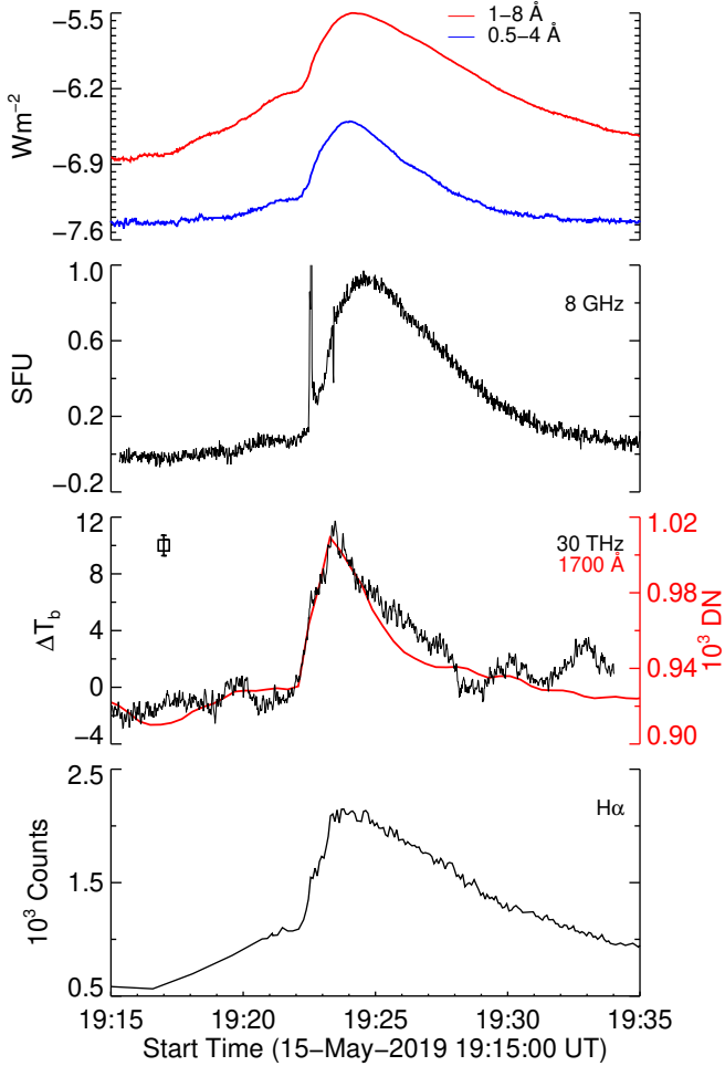
Fig. 5. Temporal evolution at selected wavelengths. From top to bottom: GOES soft X-rays 1–8 and 0.5–4 Å, EOVSA 8 GHz, AR30T mid-IR (30 THz), AIA 1700 Å and HASTA H \alpha . The error bar shown at the top left of the 30 THz plot corresponds to 1\sigma uncertainty in \Delta T_b . The sharp peak visible in the 8 GHz curve during the impulsive phase of the flare extends up to \sim 3 SFU. SFU = solar flux unit.
