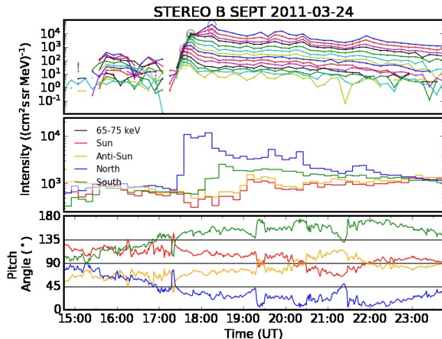
Fig. 2. Solar energetic electron observations by SEPT aboard STEREO B on 2011 Mar 24. Top panel: electron intensity in all available energy channels of one viewing direction with pre-event background subtraction, second panel: 65–75 keV intensity in the four viewing directions of SEPT, and third panel: corresponding pitch-angles based in the central pointing direction of the four telescopes.
