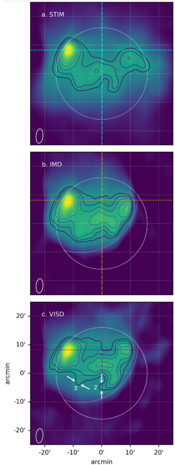
Fig. 5. Three LOFAR maps produced using three different methods. a : a CLEAN map made via standard interferometric imaging (STIM) at 10:59 UT. b : a map made by summing the Im_{diff} produced by differencing consecutive CLEAN maps, 1 min apart (IMD). c : a map made by summing the Im_{diff} , made by differencing consecutive visibility data, 1 min apart (VISD). Each map is normalised and the contours are 50–95% the max intensity. The solid white circle is the visible solar limb. The white crescent is the area not de-occulted by the moon.
