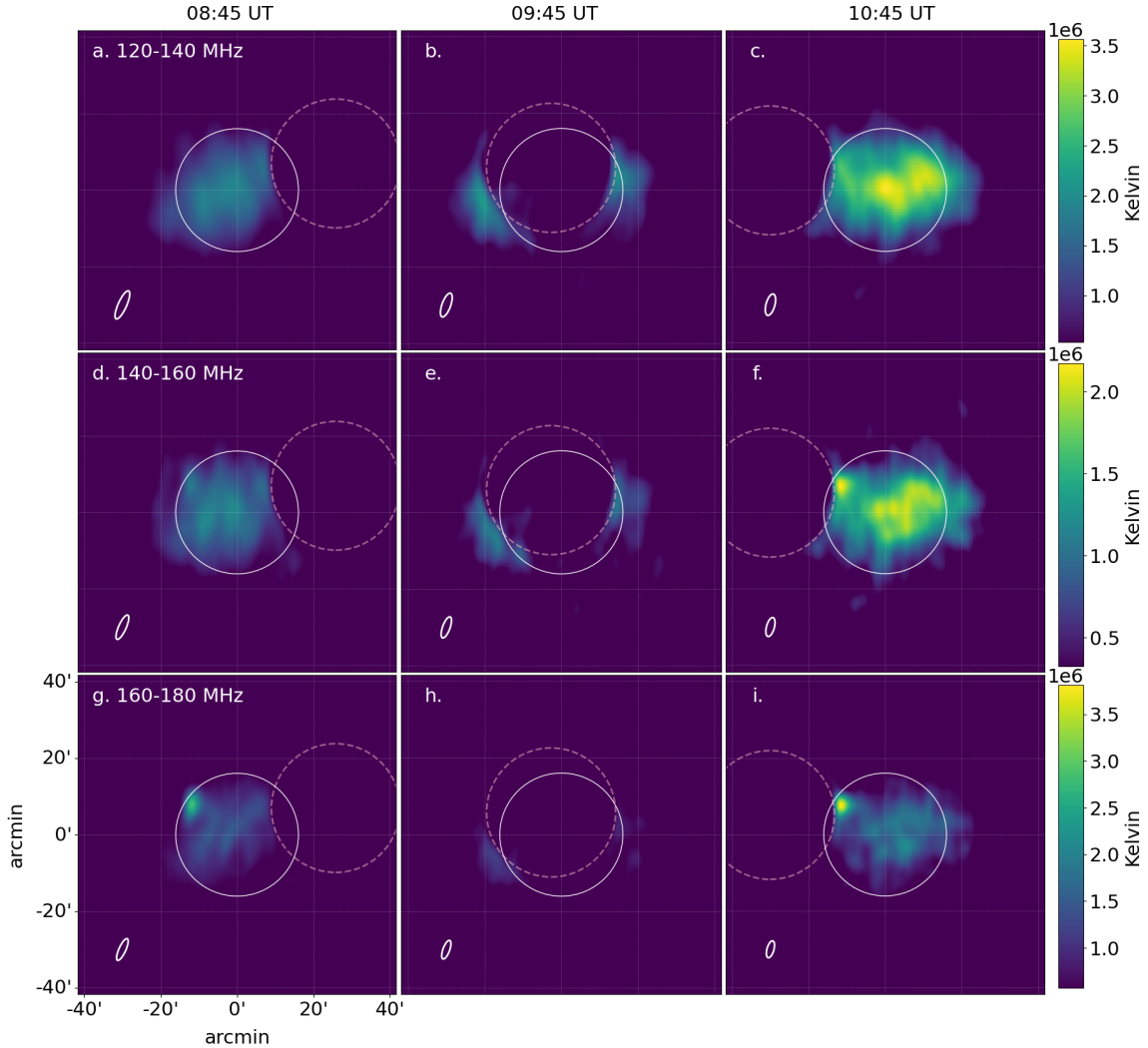
Fig. 3. LOFAR multi-frequency maps at ingress, maximum phase, and egress of the partial solar eclipse on 2015 March 20. Time increases from left to right, whereby the first column is 08:45 UT, the second column is 09:45 UT, and the third column is 10:45 UT. Frequency increases from top to bottom of the grid. The top row is the 120–140 MHz multi-frequency band, the middle row is the 140–160 MHz multi-frequency band, and the bottom row is the 160–180 MHz multi-frequency-band. In each image, the solid white circle is the visible solar limb and the pink dashed outline is the lunar limb. The white ellipse in the bottom left corner of each image is representative of the beamsize.
