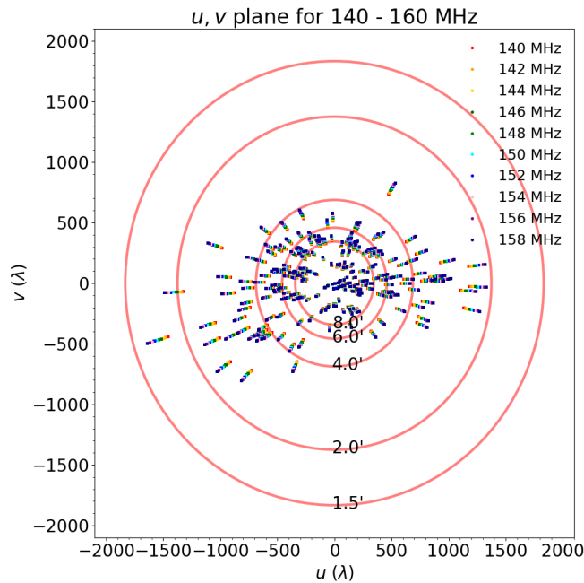
Fig. 2. u, v coverage for the multi-frequency band 140–160 MHz. Each of the coloured points on the u, v plane correspond to a different frequency observed for a given baseline. A series of red rings illustrate an example of the baselines which contribute to achieving a particular angular resolution for 140 MHz, i.e. the longer baselines are responsible for resolving the smaller structure.
