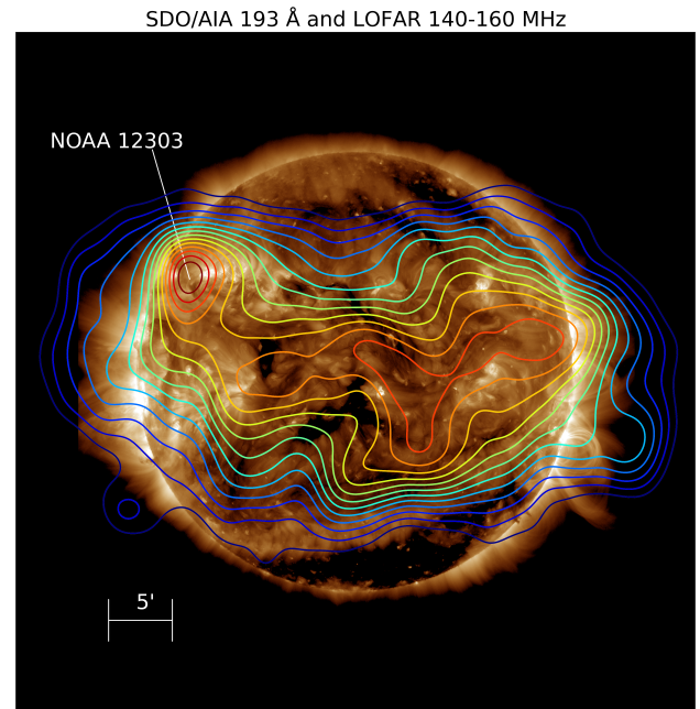
Fig. 1. LOFAR contours 50–95% (blue to red) of the peak intensity on top of a SDO/AIA 193 Å image. The contours are from a multi-frequency LOFAR map (140–160 MHz) and the 193 Å EUV image is from 11:05 UT, 2015 March 20.
