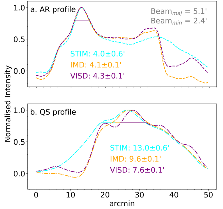
Fig. 6. Intensity slices across the bright active region (AR) emission corresponding to NOAA 12303 (---) and the quiet Sun (QS) emission (---). The profile colours correspond to the horizontal and vertical, coloured, dashed lines in Figs. 5a–c. The widths have been determined for the tallest peak, in each profile, as is labelled above.
