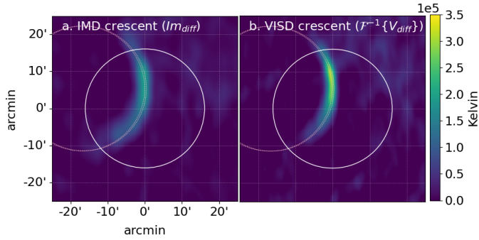
Fig. 4. Demonstration of two different approaches to the lunar de-occultation technique. a : contains the results from differencing two CLEAN maps via the image-differencing (IMD) method, i.e. Im_{diff} . b : output when the visibility data are differenced first before CLEANing, as per the visibility-differencing (VISD) method, i.e. F^{-1}\{V_{diff}\} . In both a and b , the differenced data are 1 min apart. The solid white circle is the visible solar limb and the dashed pink circle is the visible lunar limb.
