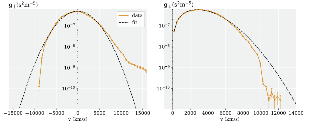
Figure 3. An example of a core fit to g(v_{\parallel}, v_{\perp}) , shown with the parallel (left), and the perpendicular (right) cut through electron VDF multiplied by v_{\perp} . Error bars represent the standard error for Poisson counting ( \sqrt{N} ). An example is taken from simulation run MC at the radial distance of 35 R_S . VDF, velocity distribution function.
