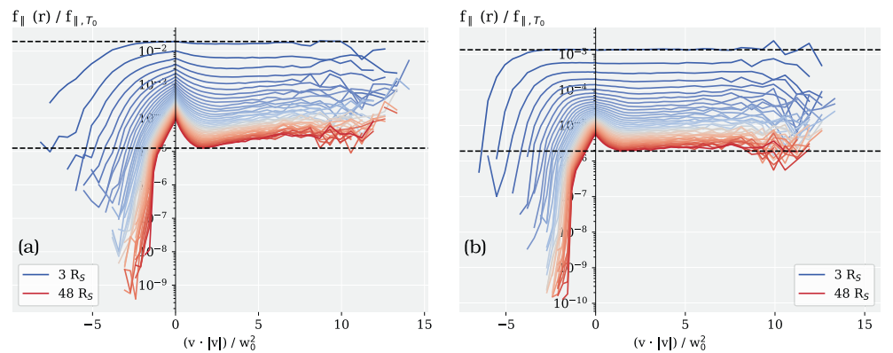
Figure B1. Electron VDFs, integrated along the \perp direction ( f_{||} ), for different radial bins, normalised with a Maxwellian VDF with the temperature T_{e,bot} . X-axis represents velocity ( v ) multiplied with its absolute value in the units of square of thermal velocity of the electron VDF at the bottom boundary ( w_0^2 ). Radial distance is presented in color spanning from blue closer to the Sun to red at the top boundary. Presented data is from the run HC (left) and run LC (right). VDF, velocity distribution function.
